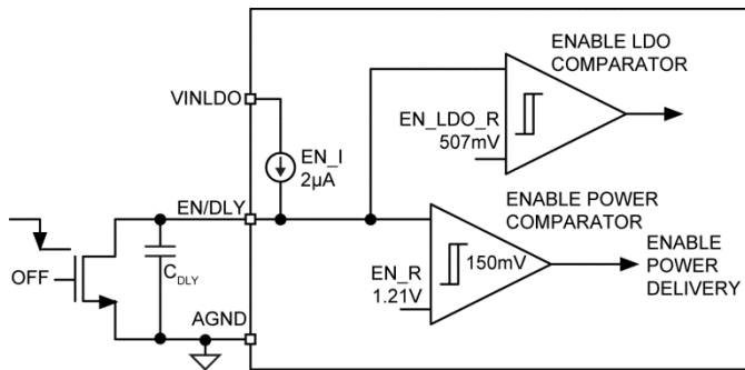
Figure 4. Programmable Start-Up Delay Function
