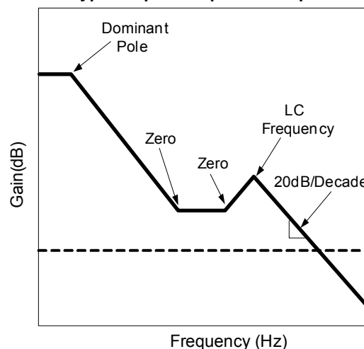
Type III Open Loop Gain Response
