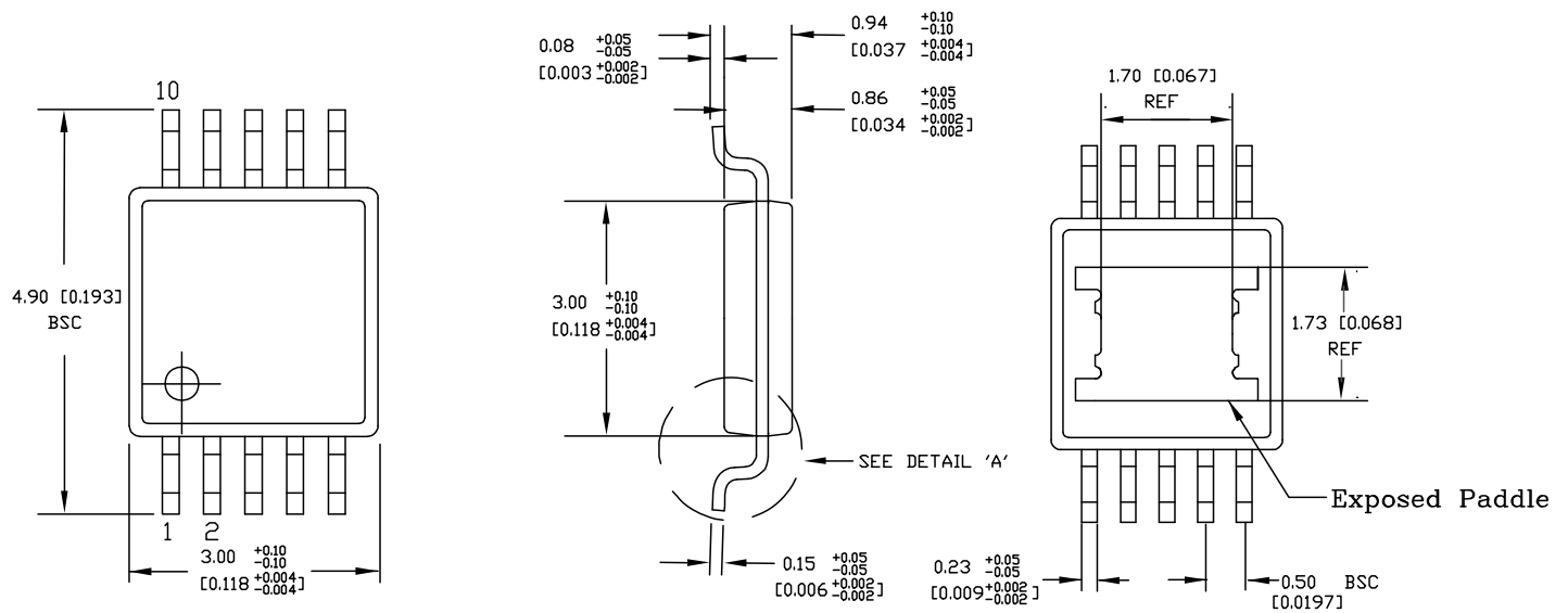
TOP VIEW
