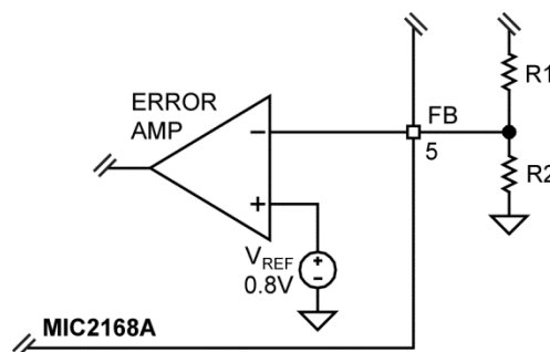
Figure 2. Voltage-Divider Configuration
