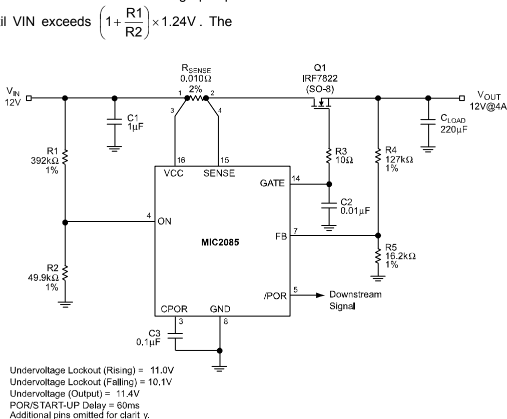
Figure 7. Higher UVLO Setting
