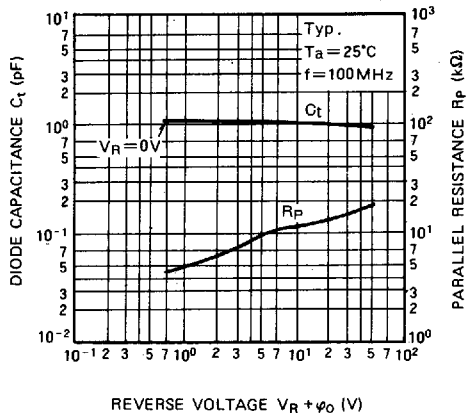
TYPICAL PERFORMANCE DATA DIODE CAPACITANCE VS. REVERSE VOLTAGE CHARACTERISTICS
