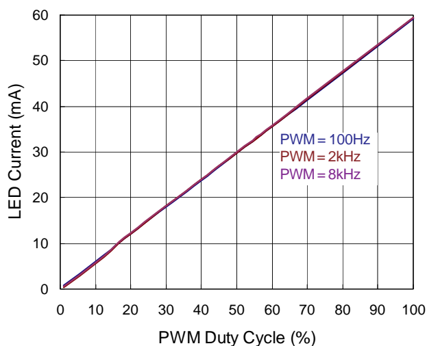
PWM Duty Cycle vs. LED Current
