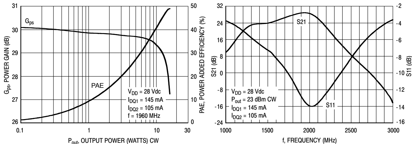
Figure 15. Power Gain and Power Added Efficiency versus Output Power
