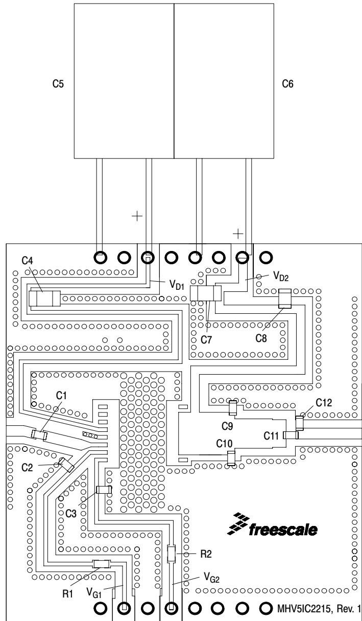
Figure 13. MHV5IC2215NR2 Test Circuit Component Layout
