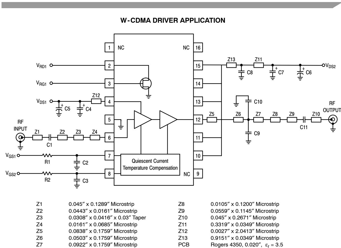
Figure 3. MHV51C2215NR2 Test Circuit Schematic
