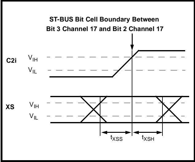
Figure 23 - XS Timing
