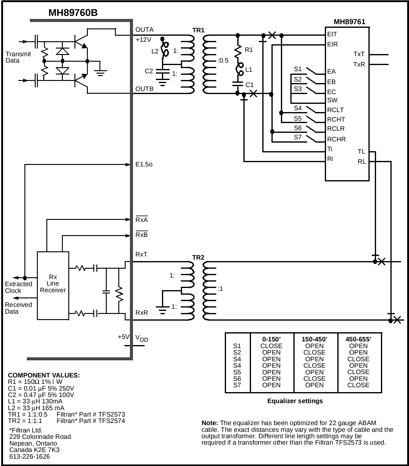
Figure 6 - Input/Output Configuration
