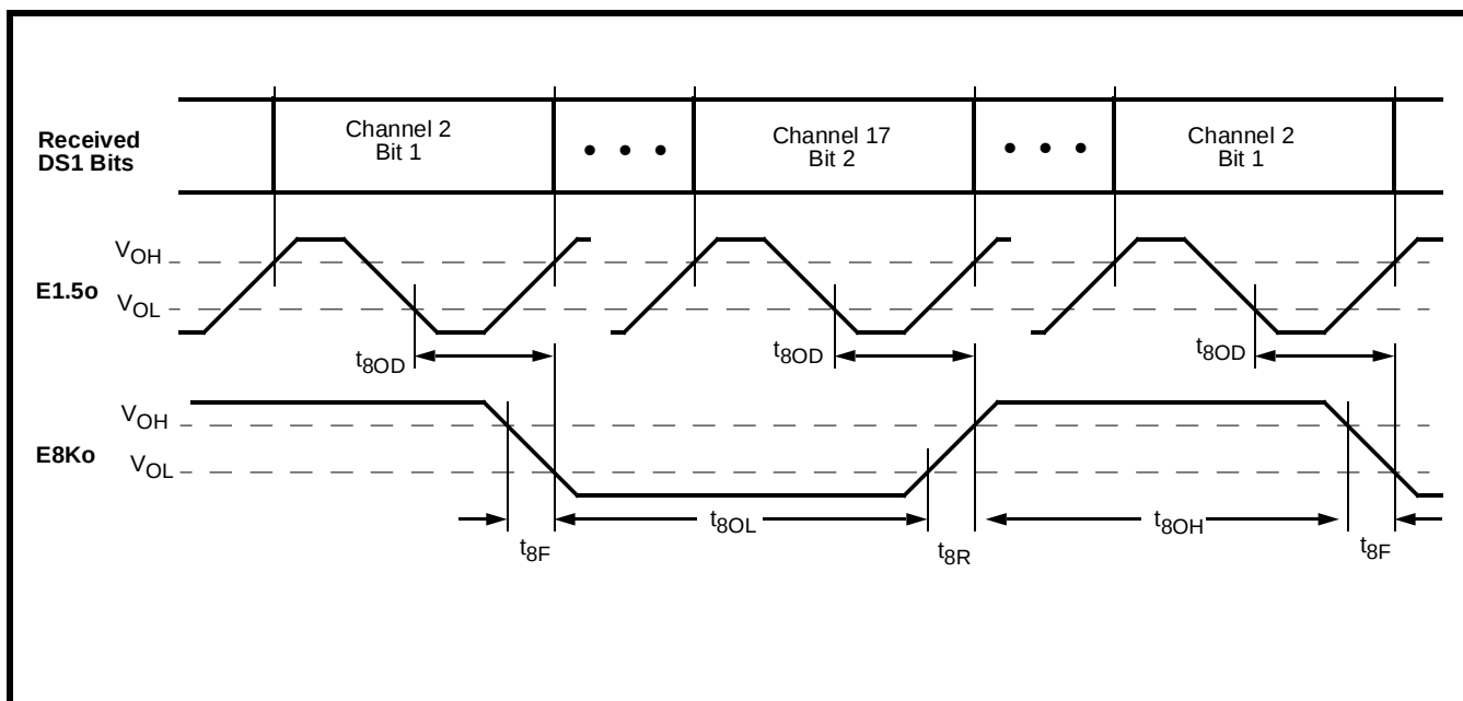
Figure 25 - E8Ko Timing
