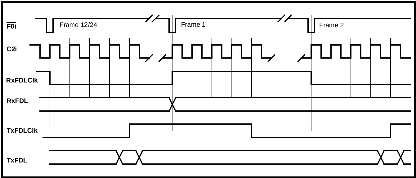
Figure 28 - Clock & Frame Alignment for Rx FDL and Tx FDL
