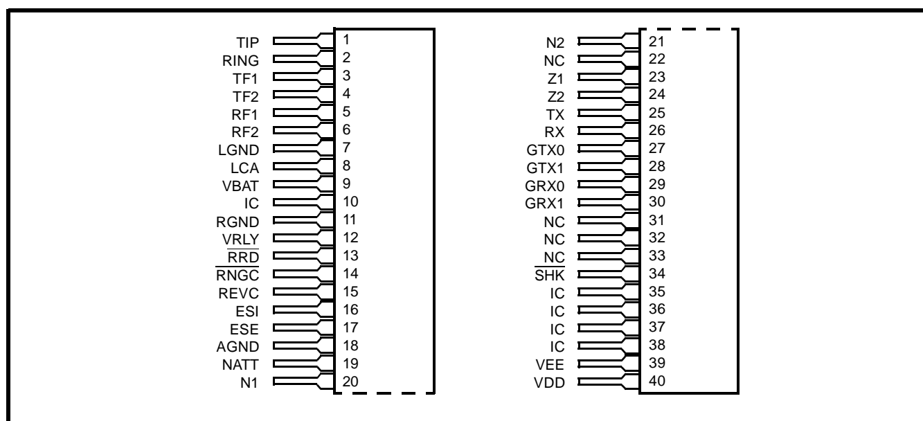
Figure 2 - Pin Connections
