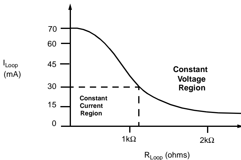
Graph 1 - I_{Loop}/R_{Loop} Characteristics
