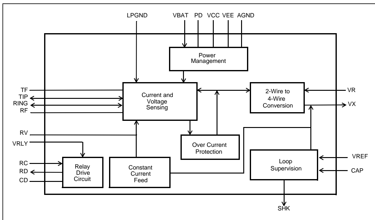
Figure 1 - Block Diagram
