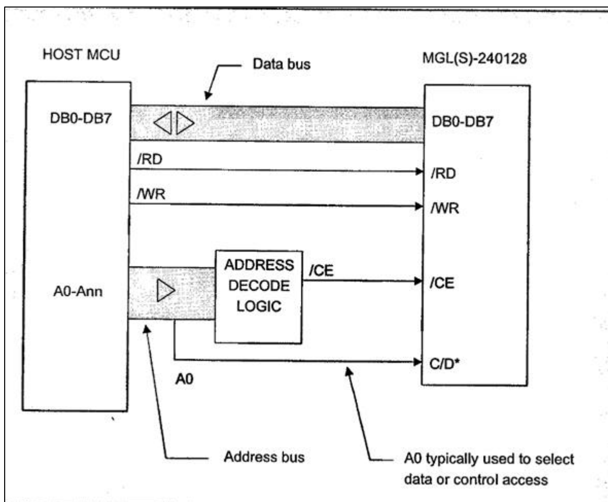
Figure 1: Typical hardware interfacing scheme
