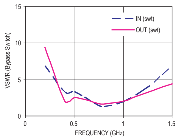
Figure 19. LNA off (Switch on) VSWR vs Frequency
