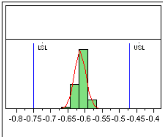
Figure 2. V_{ref} @ 3V 10mA, LSL=-0.75, Nominal=-0.61, USL=-0.47
