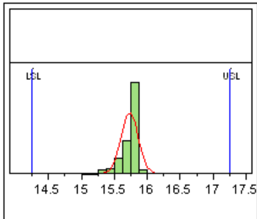
Figure 4. Gain @ 0.6GHz 3V 10mA, LSL=14.25, Nominal=15.70, USL=17.25
