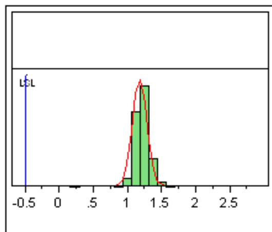
Figure 5. IIP3 @ 0.6GHz 3V 10mA, LSL=-0.5, Nominal=1.1
