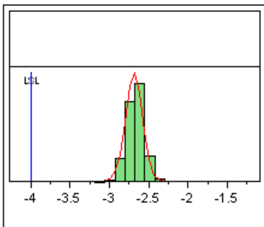
Figure 6. I_{L\_bypass} @ 0.6GHz 3V 0mA, LSL=-4.0, Nominal=-2.6
