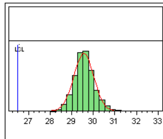
Figure 7. IIP3\_bypass @ 0.6GHz 3V 0mA, LSL=26.5, Nominal=29.5
