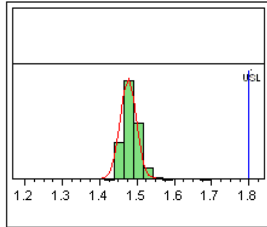
Figure 3. NF @ 0.6GHz 3V 10mA, Nominal=1.5, USL=1.8
