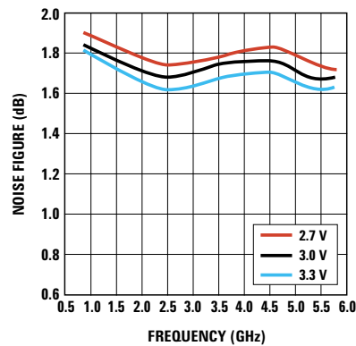
Figure 20. Noise figure (50 \Omega ) vs. frequency and voltage.
