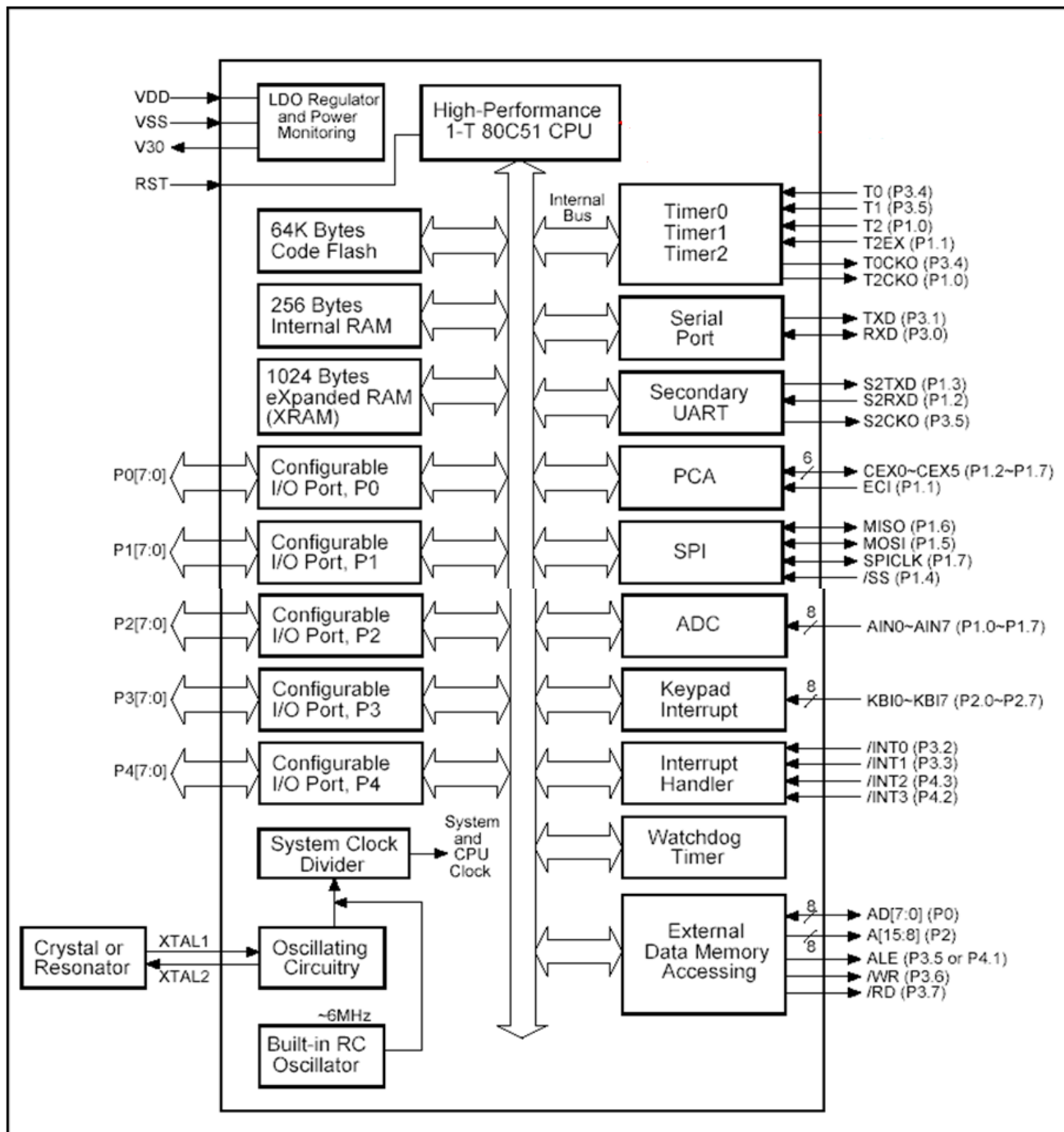
Figure 3-1. 方框图
