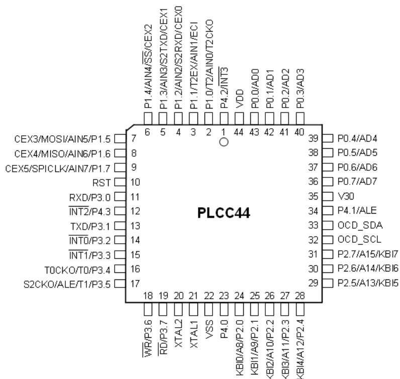
Figure 4-2. 引脚结构: 44-Pin PLCC
