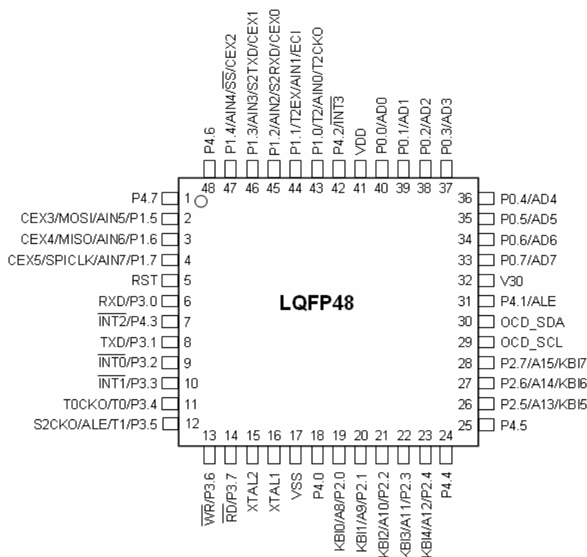
Figure 4-4. 引脚结构: 48-Pin LQFP
