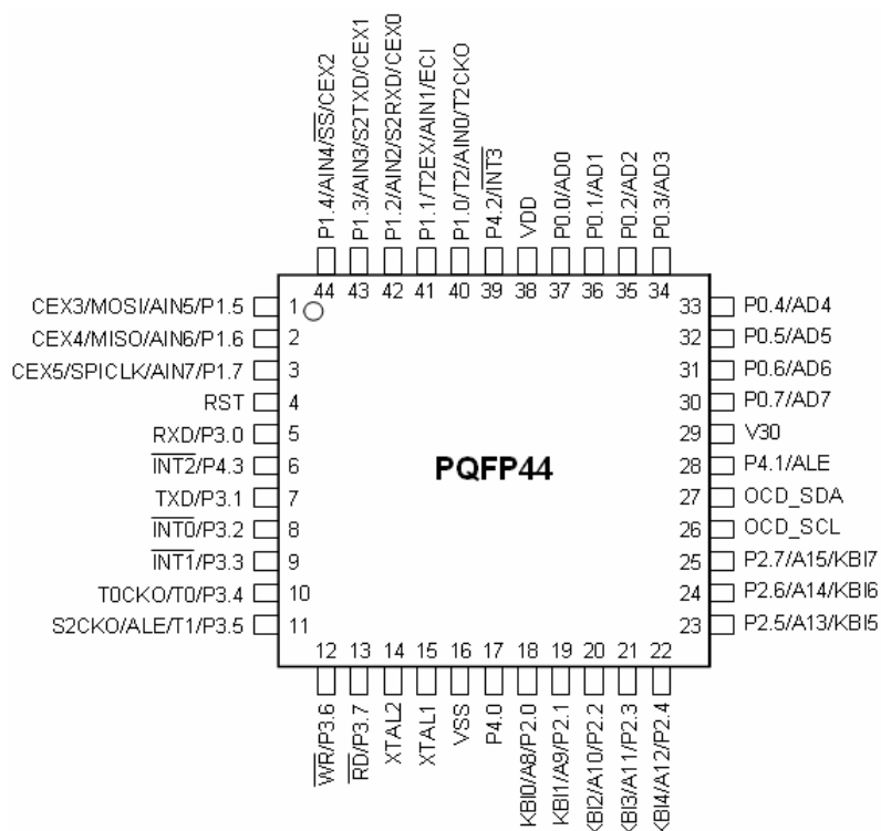
Figure 4-3. 引脚结构: 44-Pin PQFP
