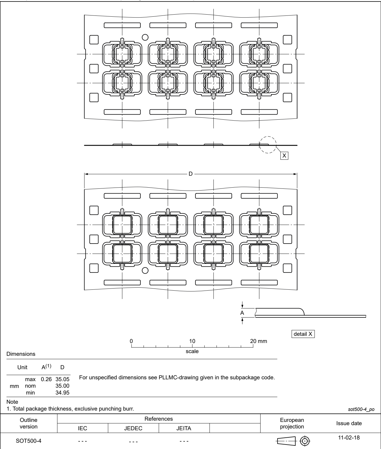
Figure 23. Package outline SOT500-4
