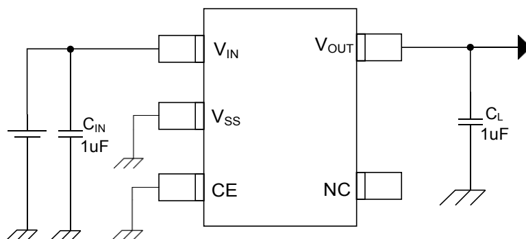
Fig3. ME6511H series
