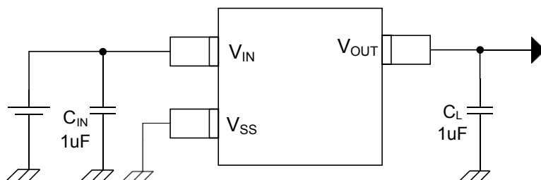
Fig1. ME6511A series
