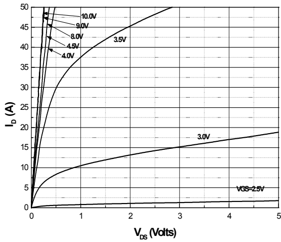
Fig.1 On-Region Characteristics
