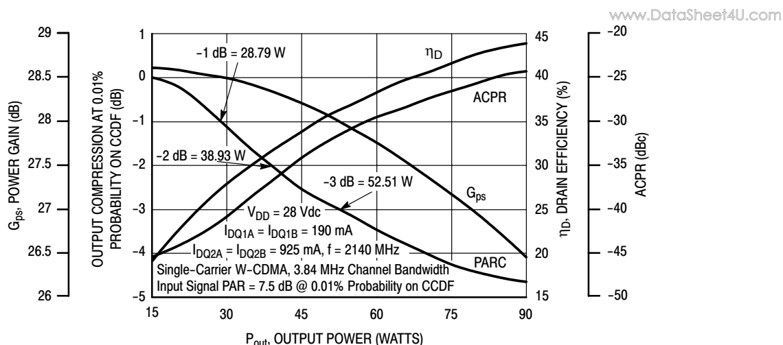
Figure 10. Output Peak-to-Average Ratio Compression (PARC) versus Output Power
