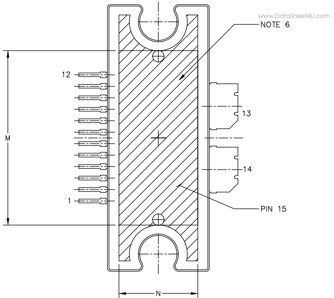
VIEW Y-Y
