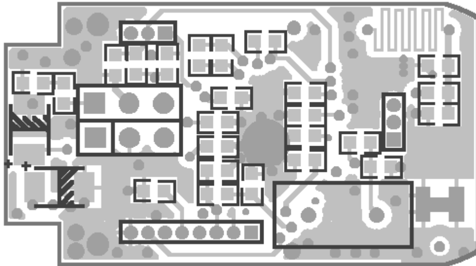
Figure 3: Bottom Layer Layout
