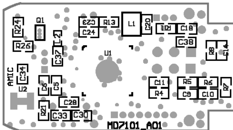
Figure 4: Top Layer Placement
