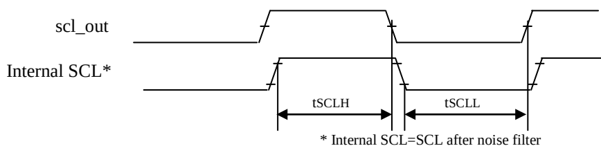
Figure 18-3 tSCLH/tSCLL Timing definition
