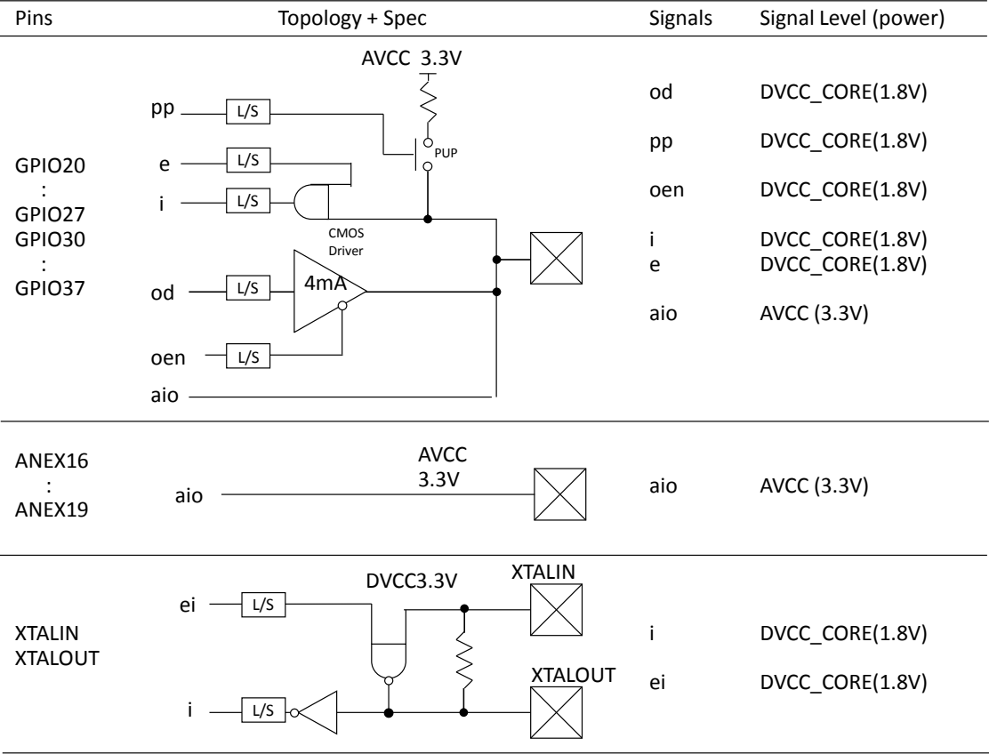
Figure 8-1 GPIO/PIN Structures
