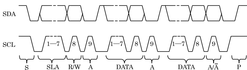
Figure 18-7 I2C bus timing
