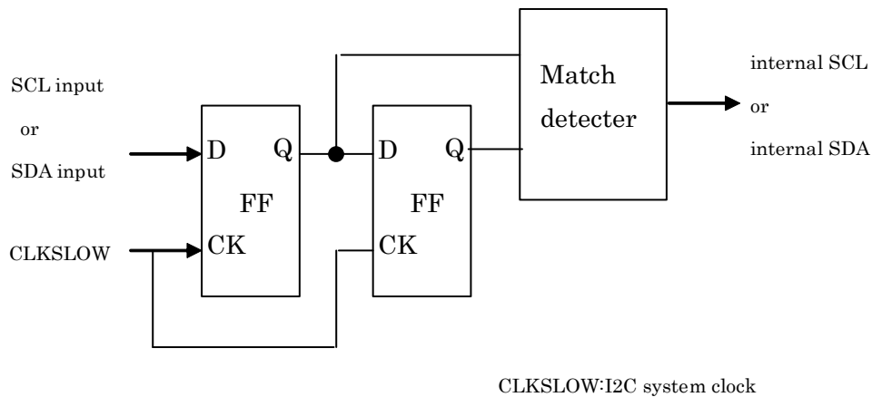
Figure 18-12 Block Diagram of the noise filter
