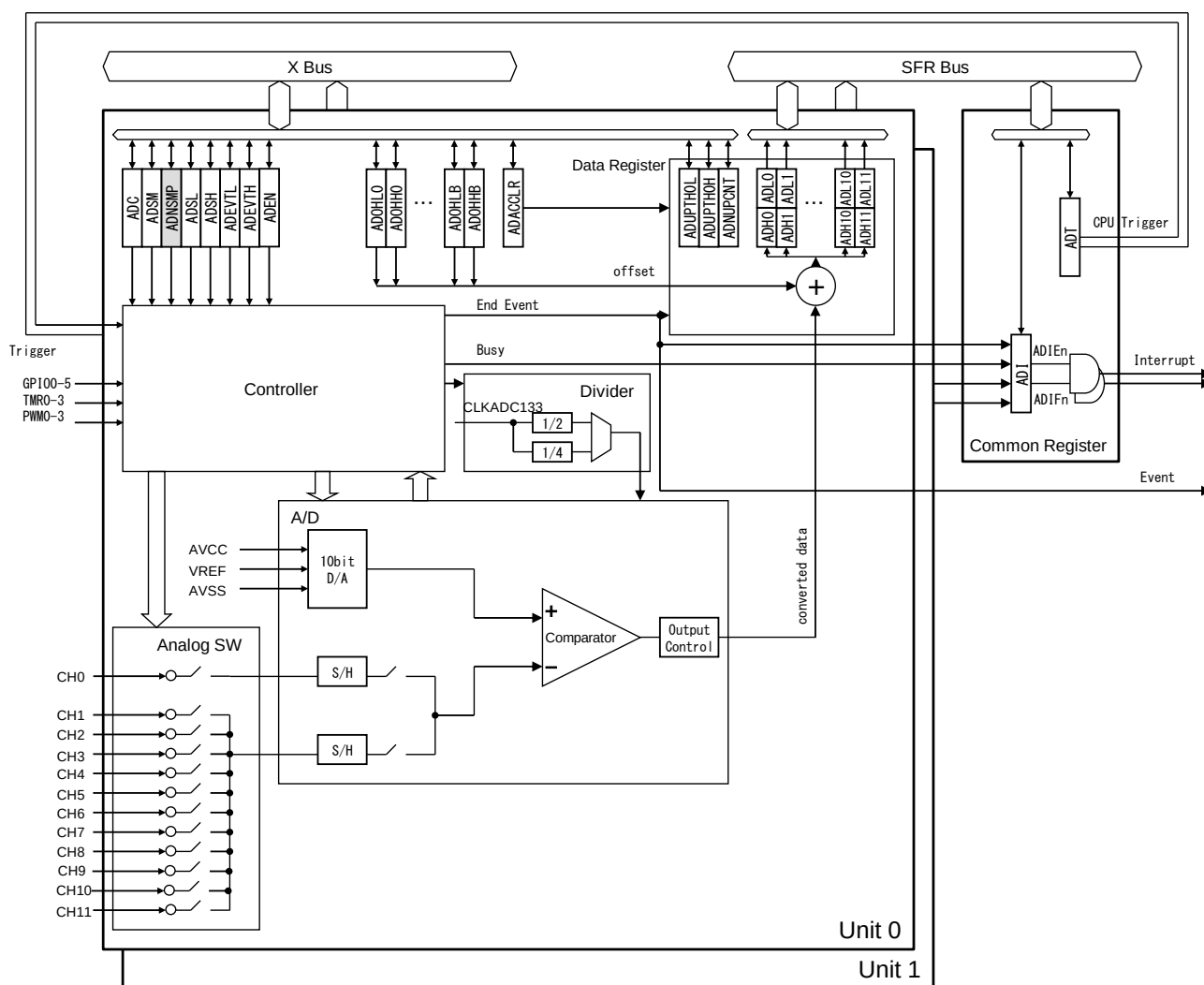
Figure 21-1 Block Diagram of 10bit ADC
