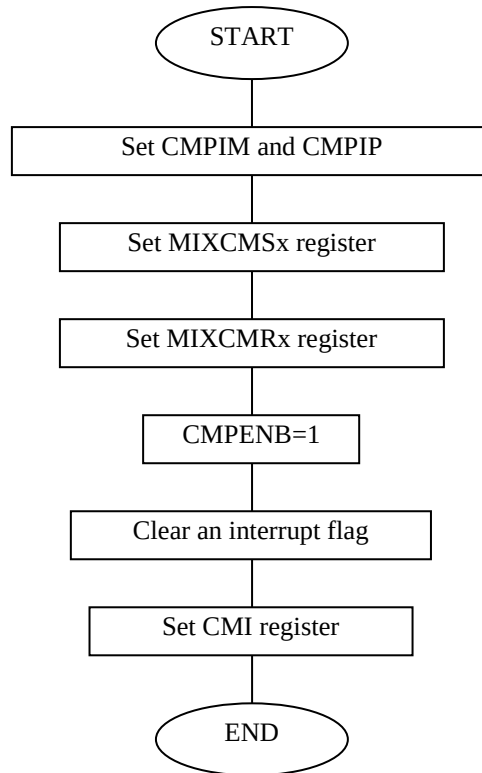
Figure 25-3 Operation flowchart
