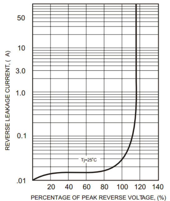
FIG.4-TYPICAL REVERSE CHARACTERISTICS
