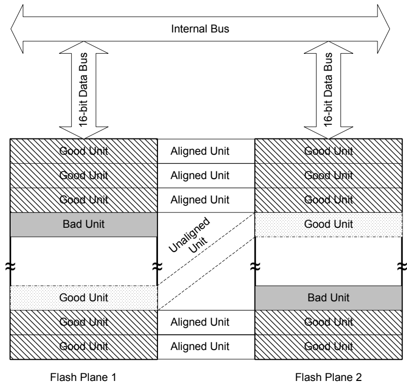
Figure 10: Unaligned Multi-Plane Access
