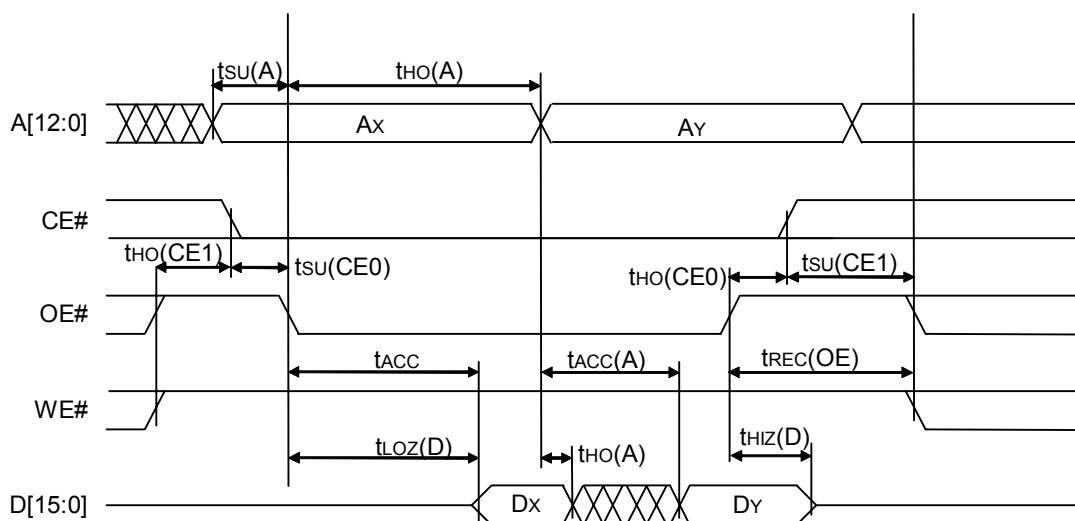
Figure 24: Standard Interface Read Cycle Timing – Asynchronous Boot Mode
