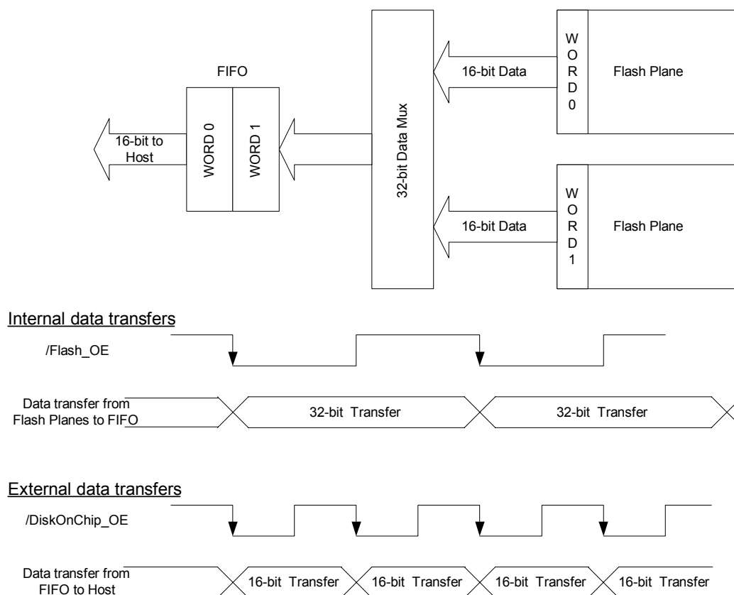
Figure 11: MultiBurst Operation
