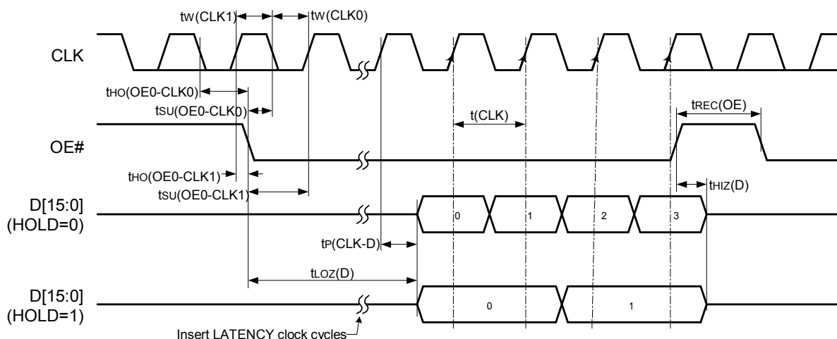
Figure 28: MultiBurst Read Timing
