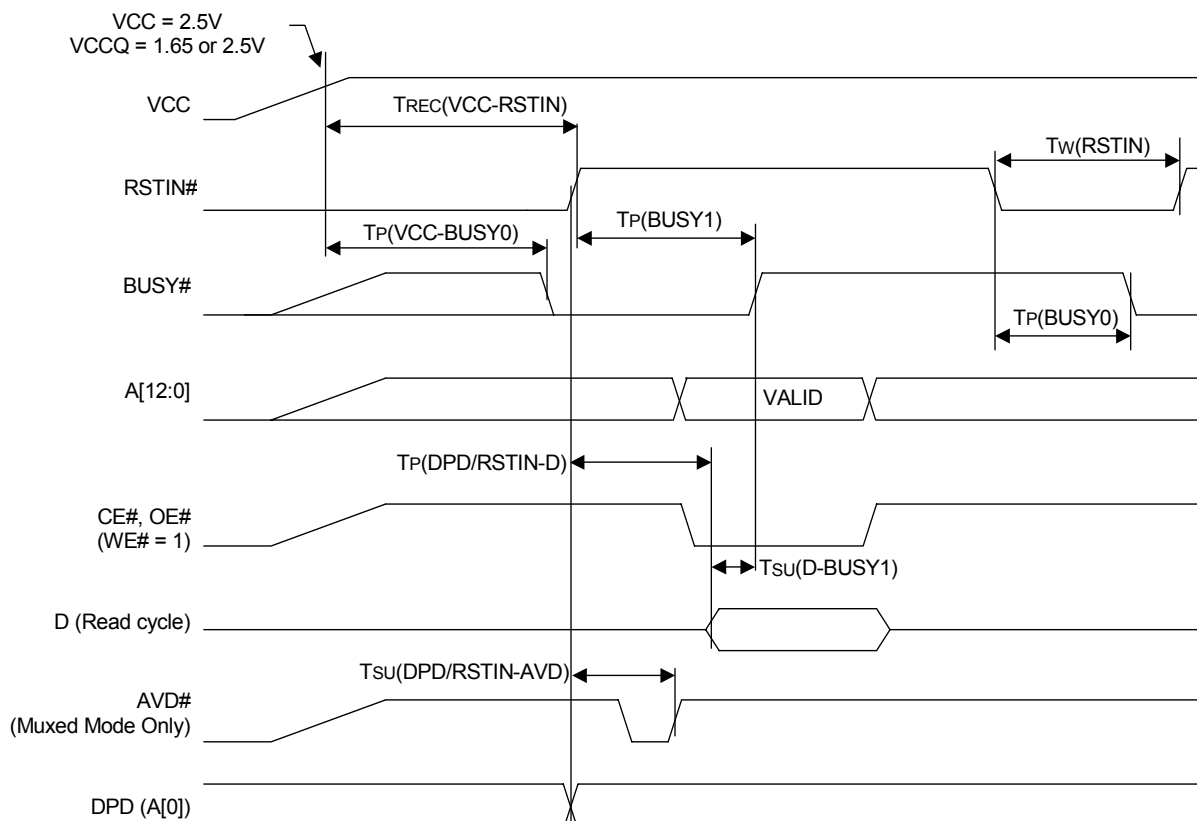
Figure 29: Reset Timing
