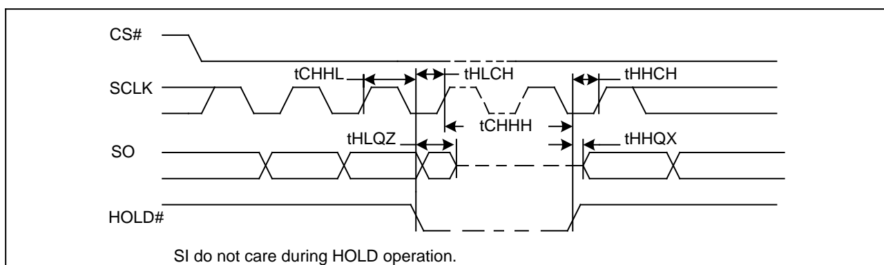
Figure49. Hold Timing
