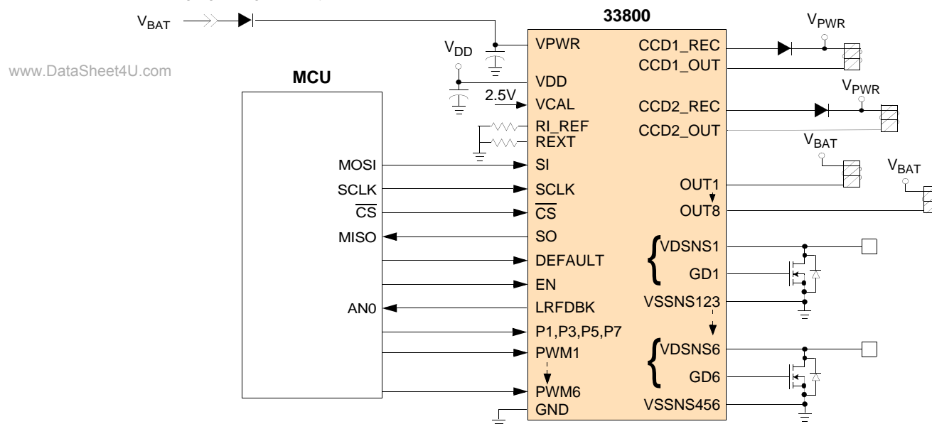
Figure 1. MC33800 Simplified Application Diagram
