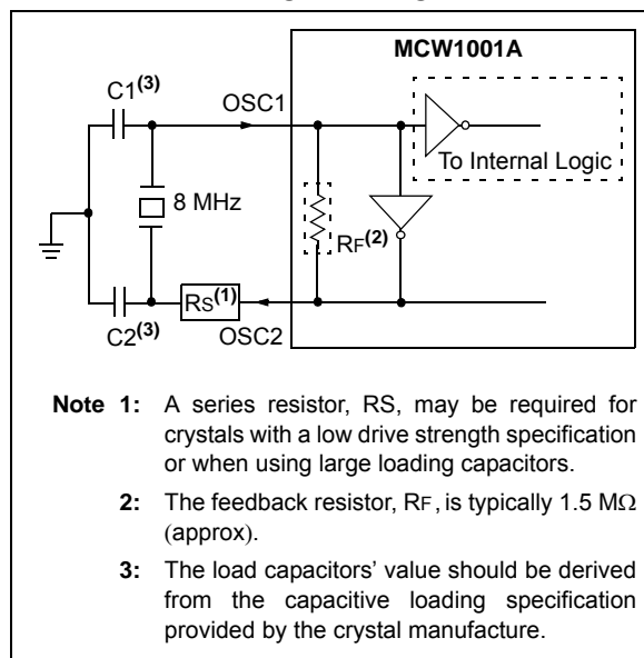
FIGURE 2-1: CRYSTAL OSCILLATOR OPERATION
