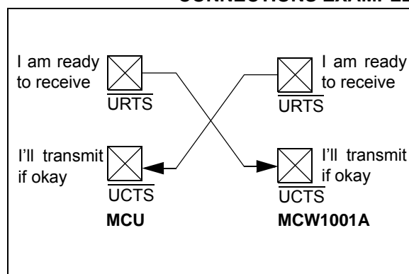
FIGURE 3-1: URTS/UCTS CONNECTIONS EXAMPLE
