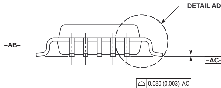
DETAIL AD
