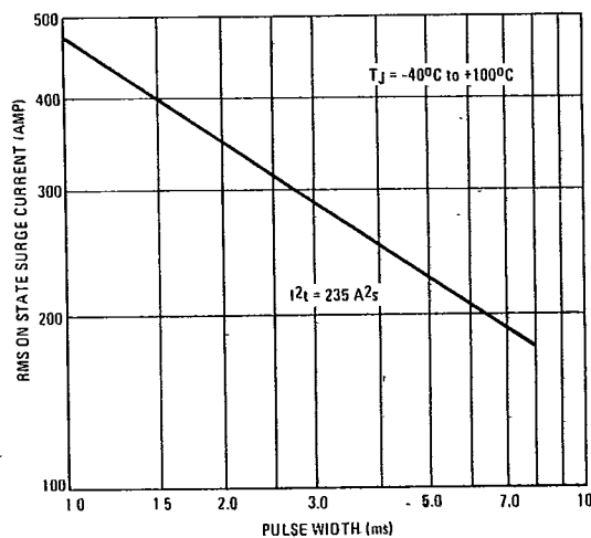
FIGURE 4 - SUB-CYCLE SURGES
