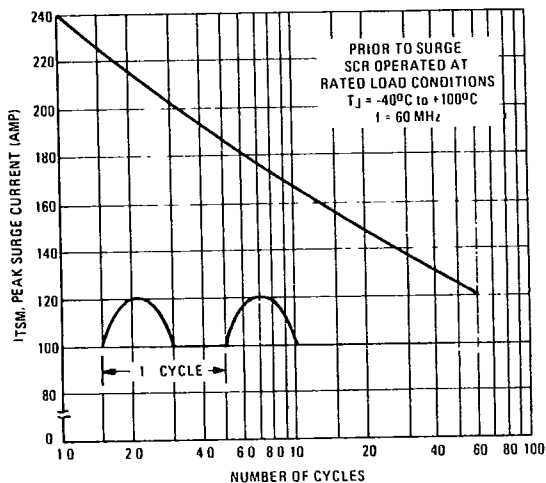
FIGURE 3 - 60 Hz SURGES
