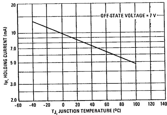
FIGURE 6 - EFFECT OF TEMPERATURE ON TYPICAL HOLDING CURRENT
