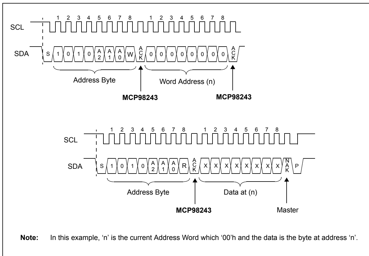
FIGURE 5-20: Timing Diagram for Random Read (See Section 4.0 "Serial Communication").
