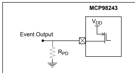
FIGURE 5-11: Active-High Event Output Configuration.
