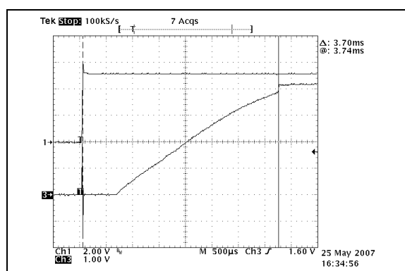
FIGURE 2-24: V_{USB} UVLO Start Delay (USB = Low).
