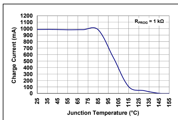
FIGURE 2-12: Charge Current ( I_{OUT} ) vs. Junction Temperature ( T_J ).
