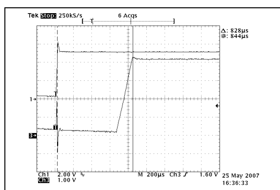
FIGURE 2-23: V_{AC} UVLO Start Delay ( I_{OUT} = 1A ).
