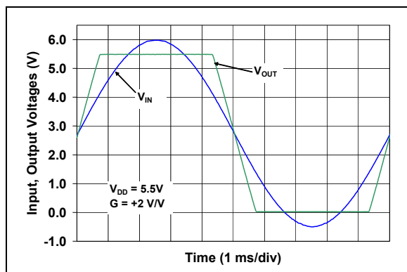
FIGURE 2-31: The MCP6286 Shows No Phase Reversal.
