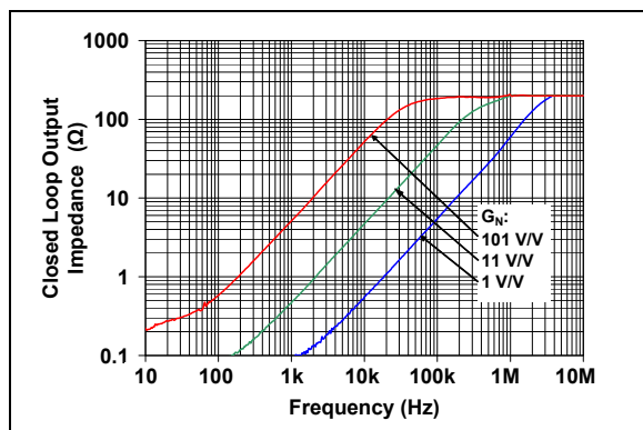
FIGURE 2-32: Closed Loop Output Impedance vs. Frequency.
