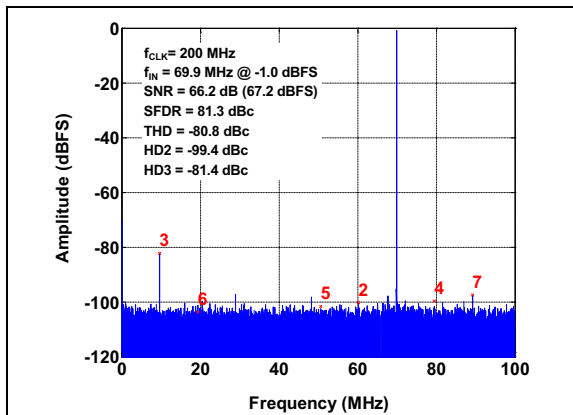
FIGURE 3-2: FFT for 69.9 MHz Input Signal: f_S = 200\text{ Mps} , A_{IN} = -1\text{ dBFS} .
