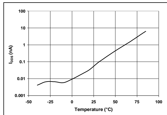
FIGURE 2-29: I_{DD5} vs. Temperature.
