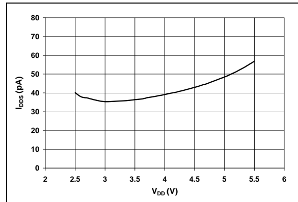
FIGURE 2-28: I_{DD5} vs. V_{DD} .
