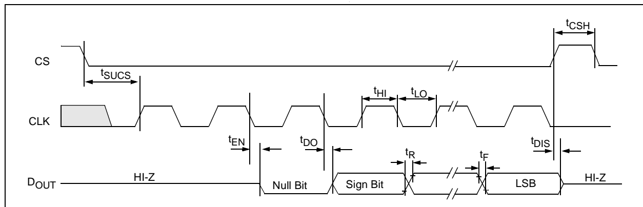
FIGURE 1-1: Timing Parameters.
