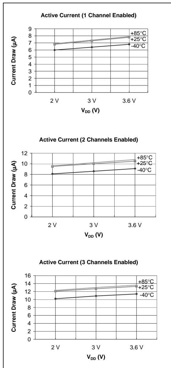
FIGURE 2-2: Typical Active Current.
