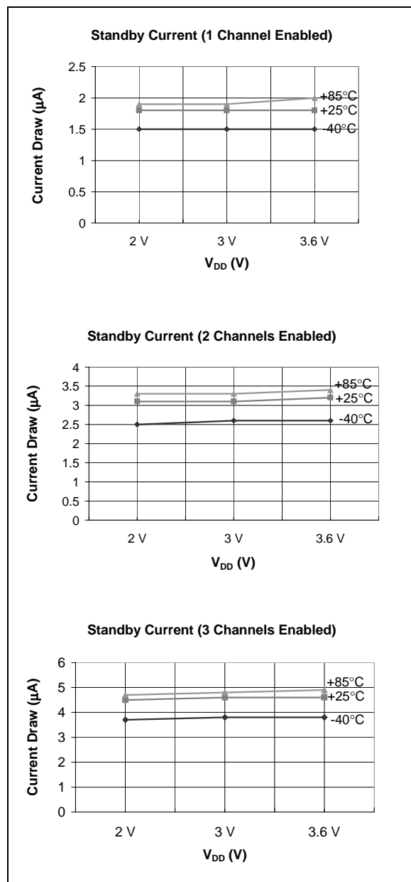
FIGURE 2-1: Typical Standby Current.
