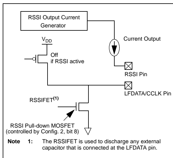
FIGURE 5-8: RSSI Output Path.
