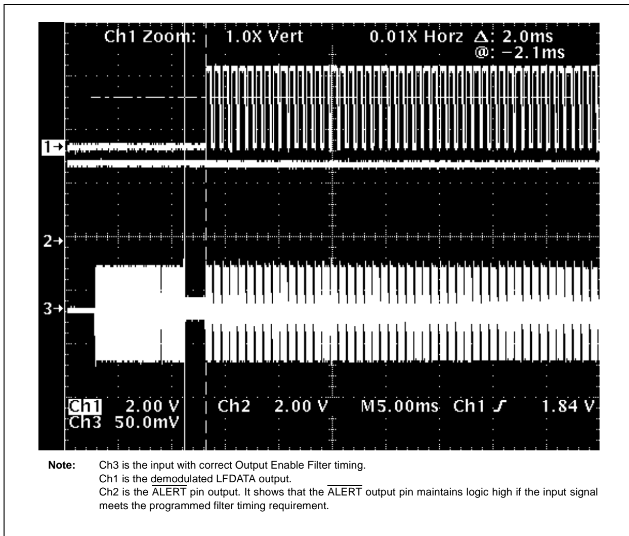
FIGURE 2-18: \overline{\text{ALERT}} Output Example: With No Parity Error and no 32 ms Alarm Timer Time-out.
