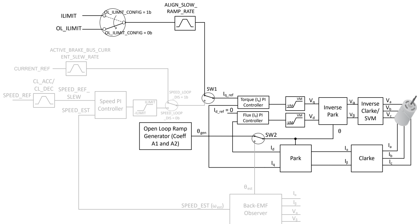
Figure 6-30. Open Loop
