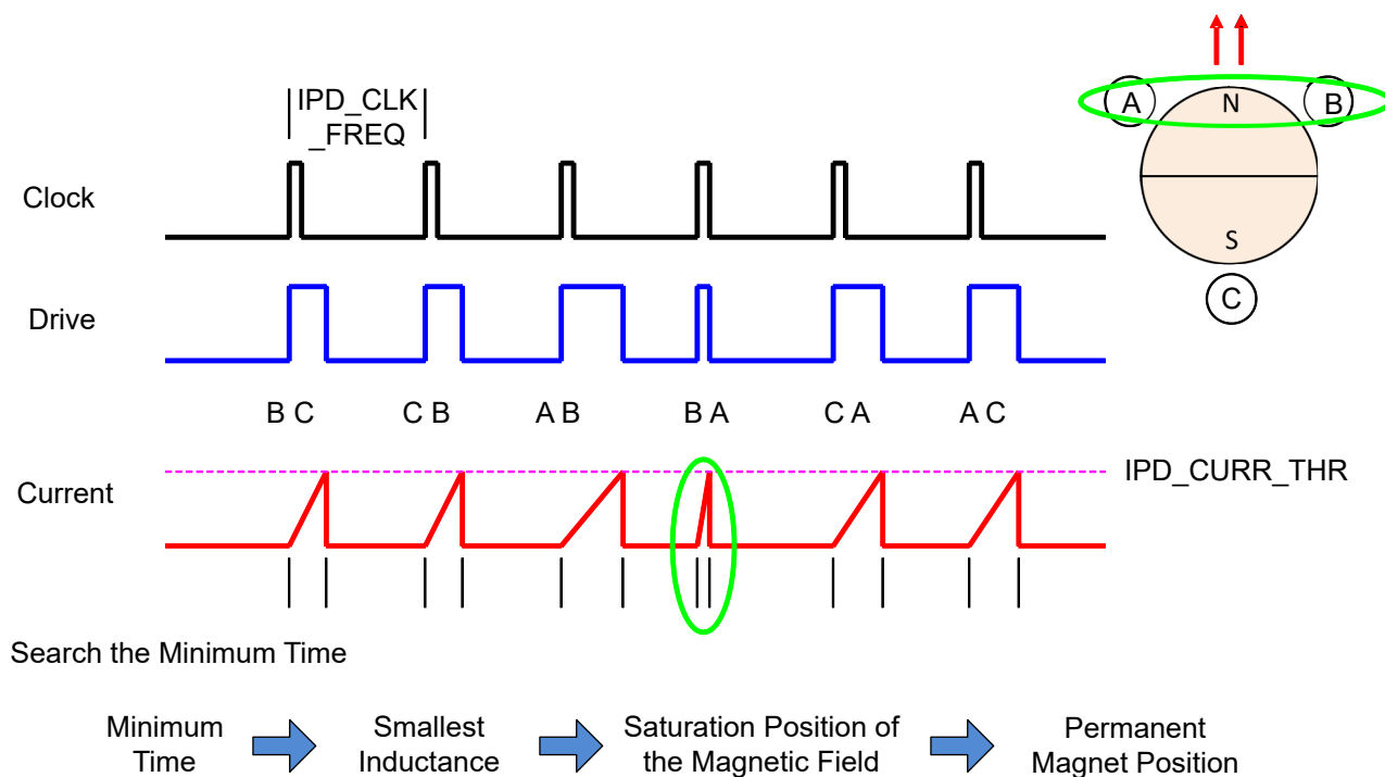
Figure 6-26. IPD Operation
