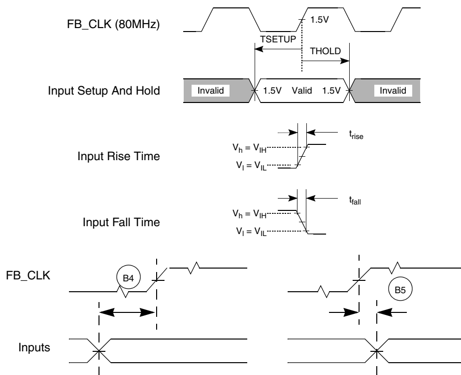
Figure 10. General Input Timing Requirements
