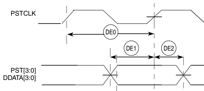
Figure 31. Real-Time Trace AC Timing
