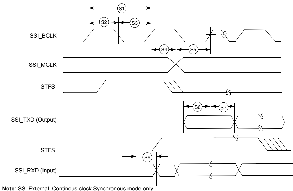
Figure 20. SSI External Continuous Clock Timing Diagram
