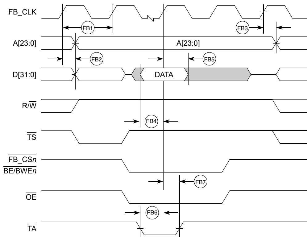
Figure 11. FlexBus Read Timing.
