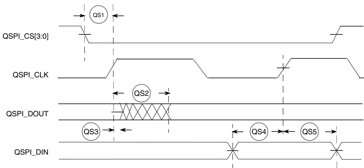
Figure 26. QSPI Timing
