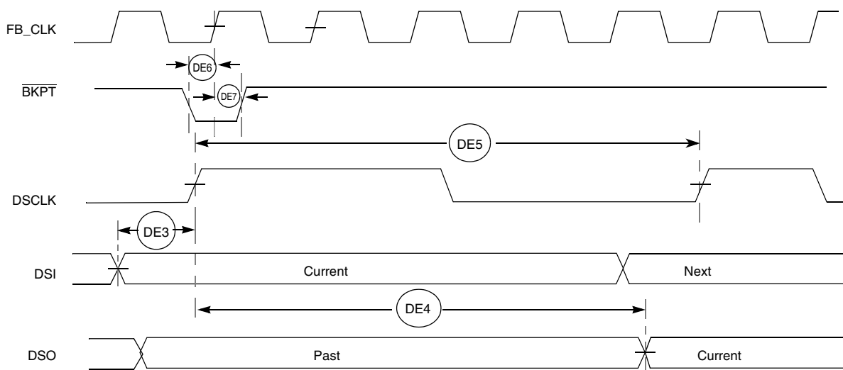
Figure 32. BDM Serial Port AC Timing
