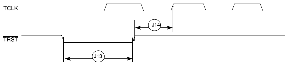
Figure 30. \overline{\text{TRST}} Timing
