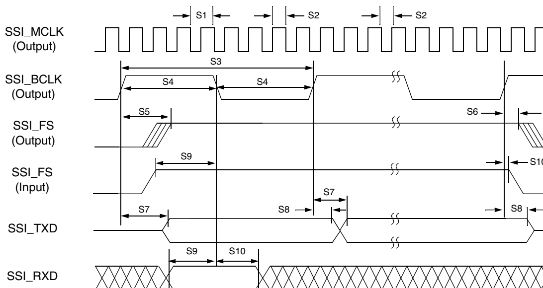
Figure 14. SSI Timing – Master Modes
