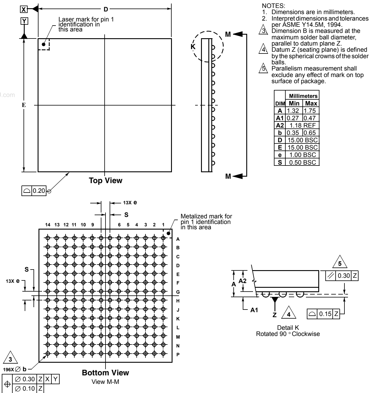
Figure 30. 196 MAPBGA Package Dimensions (Case No. 1128A-01)
