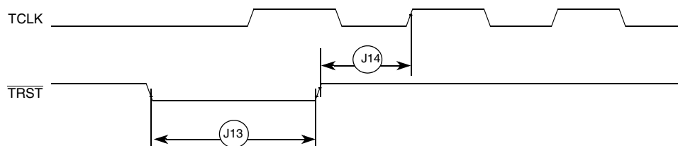
Figure 25. \overline{\text{TRST}} Timing
