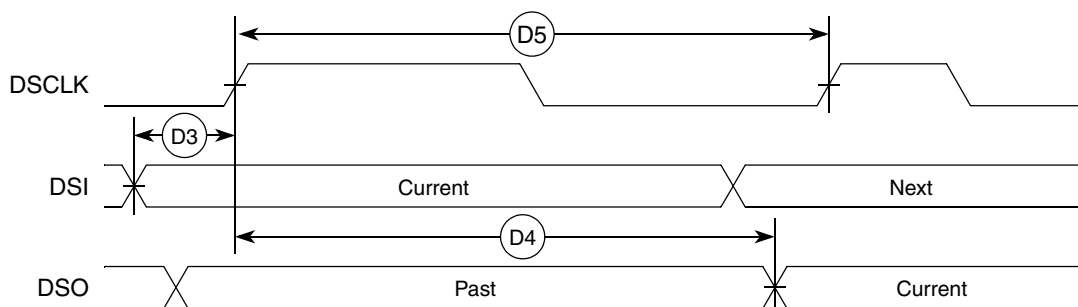
Figure 27. BDM Serial Port AC Timing
