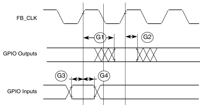
Figure 12. GPIO Timing
