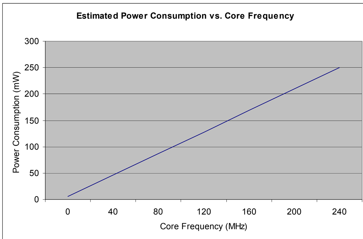
Figure 4. Estimated Maximum RUN Mode Power Consumption
