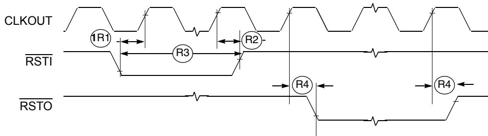
Figure 12. \overline{\text{RSTI}} and Configuration Override Timing
