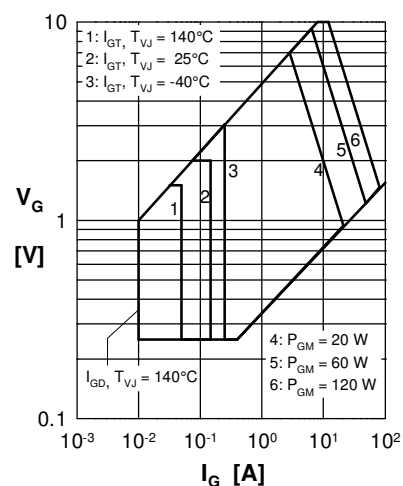
Fig. 5 Surge overload current I_{T(F)SM} : Crest value, t: duration
