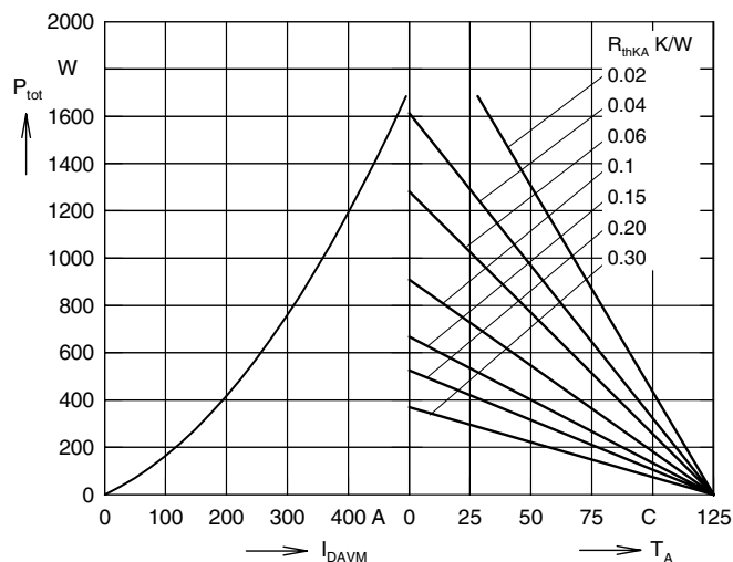
Fig. 8: Power dissipation vs. direct output current and ambient temperature (three phase rectifier bridge)
