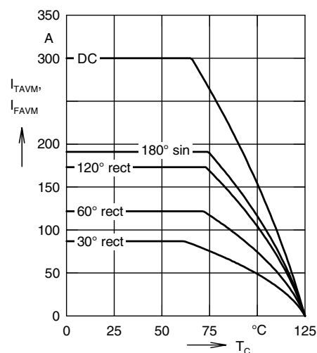
Fig. 6: Max. forward current at case temperature I_{TAVM/FAVM} = f(T_C, d)
