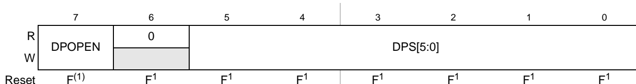
Figure 19-15. EEPROM Protection Register (DFPROT)
