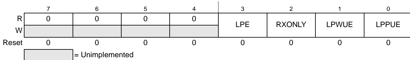
Figure 20-4. LIN Control Register (LPCR)
