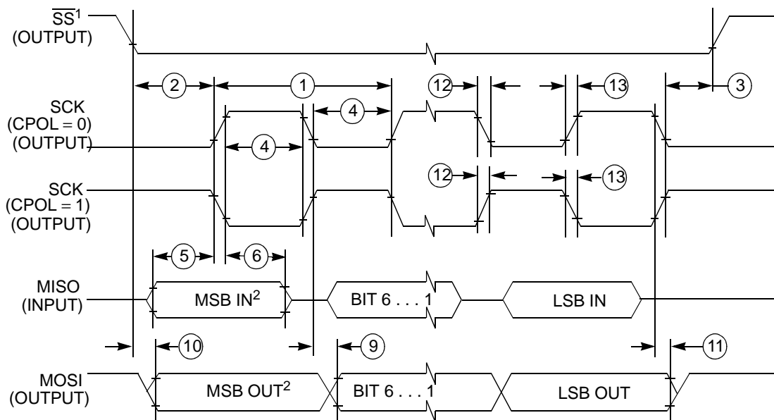
Figure M-1. SPI Master Timing (CPHA=0)
