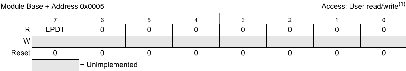
Figure 20-8. LIN Status Register (LPSR)
