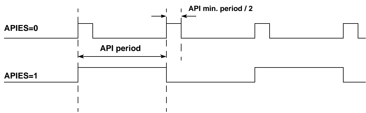
Figure 7-21. Waveform selected on API_EXTCLK pin (APIEA=1, APIFE=1)
