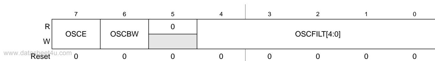
Figure 7-29. S12CPMU Oscillator Register (CPMUOSC)
