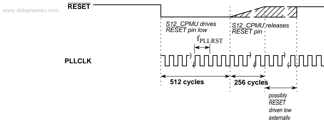
Figure 7-37. RESET Timing
