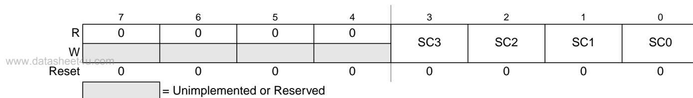
Figure 6-10. Debug State Control Register 2 (DBGSCR2)
