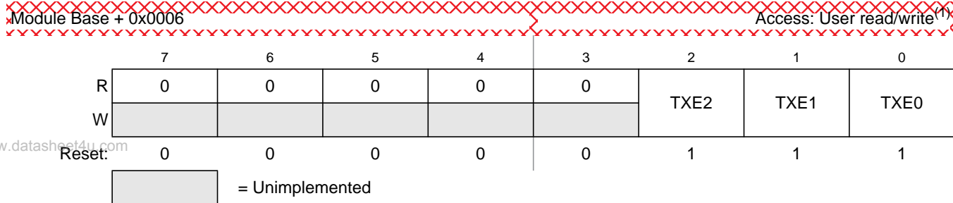
Figure 8-10. MSCAN Transmitter Flag Register (CANTFLG)
