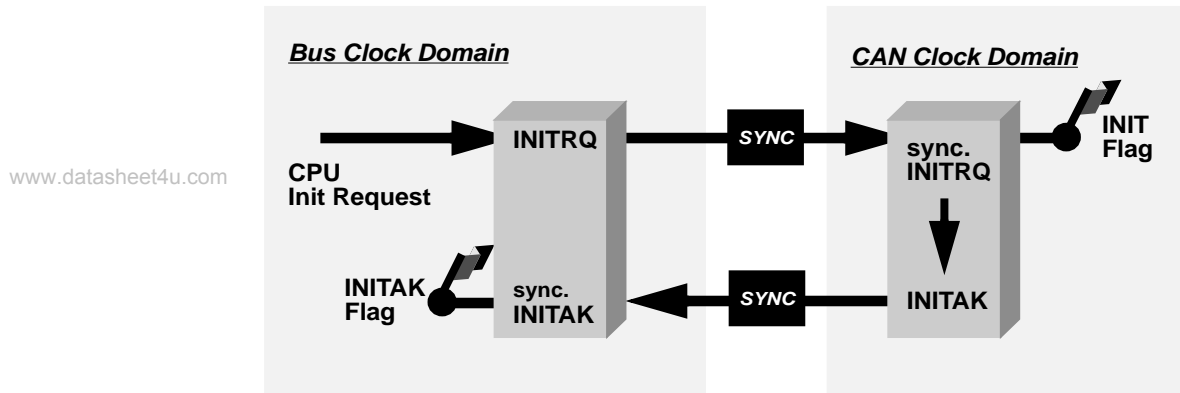
Figure 8-45. Initialization Request/Acknowledge Cycle
