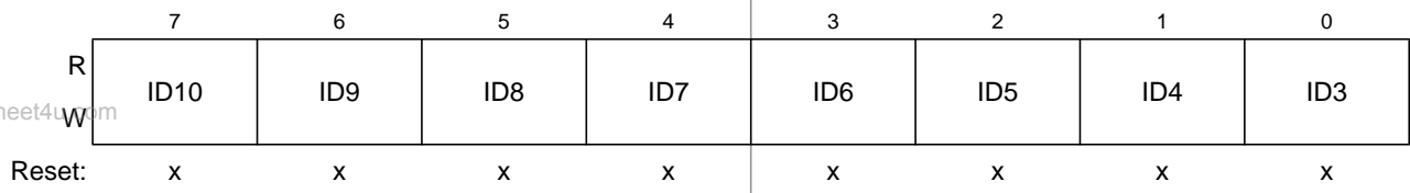
Figure 8-30. Identifier Register 0 — Standard Mapping
