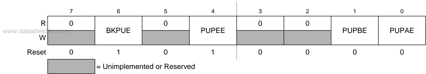
Figure 2-8. Ports ABKE, BKGD pin Pull-up Control Register (PUCR)
