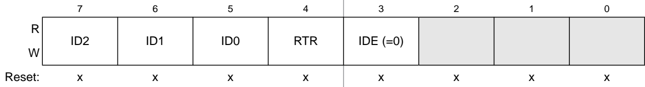
Figure 8-31. Identifier Register 1 — Standard Mapping
