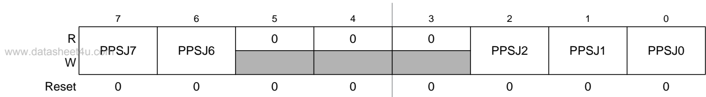
Figure 2-52. Port J Polarity Select Register (PPSJ)
