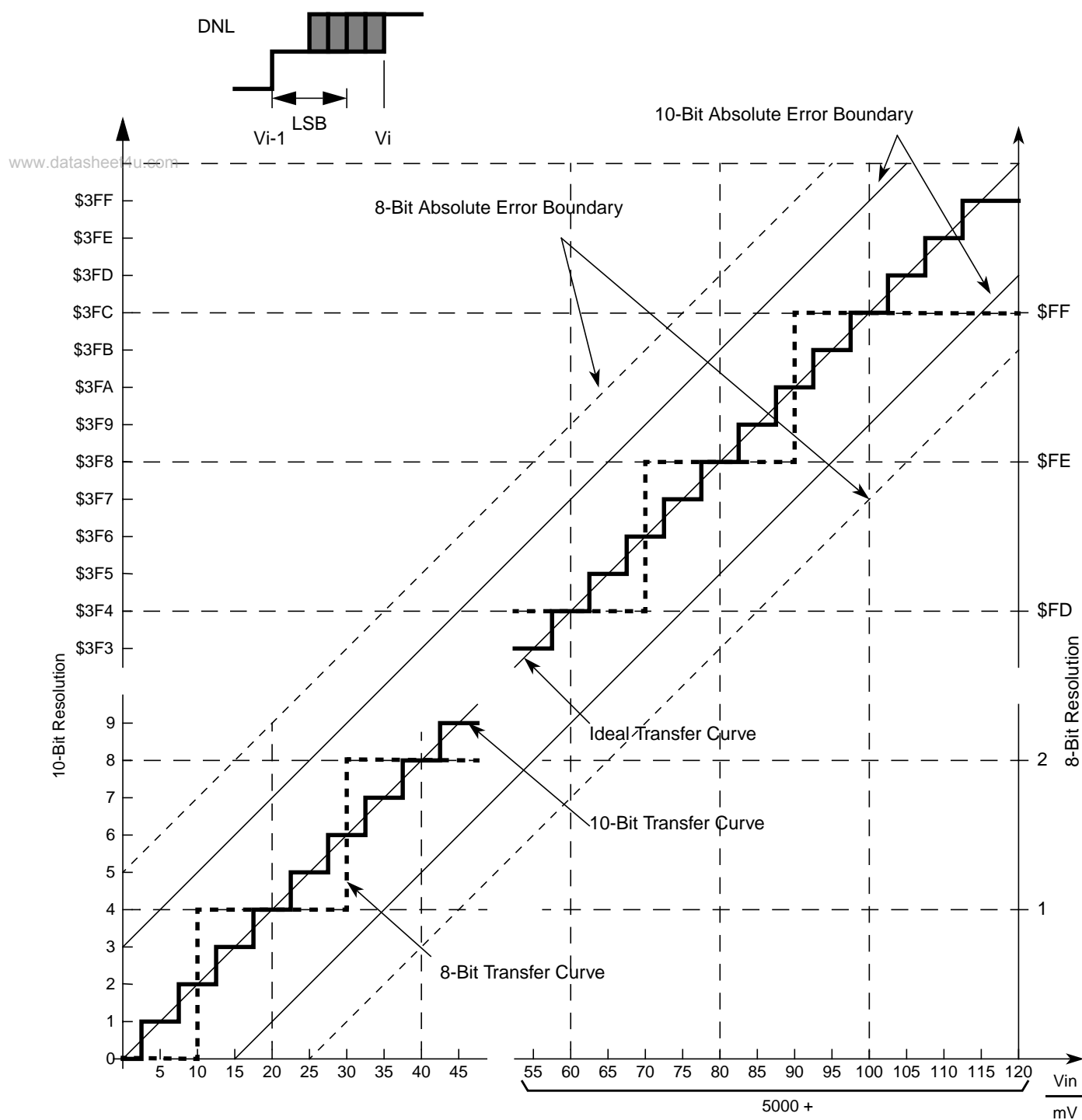
Figure A-1. ATD Accuracy Definitions
