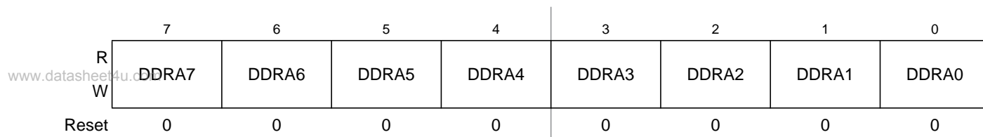
Figure 2-3. Port A Data Direction Register (DDRA)
