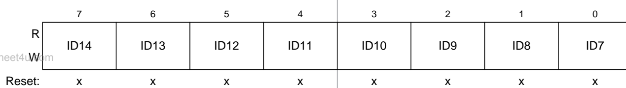
Figure 8-28. Identifier Register 2 (IDR2) — Extended Identifier Mapping
