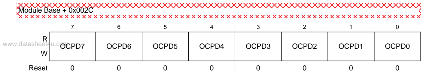
Figure 14-28. Ouput Compare Pin Disconnect Register (OCPD)
