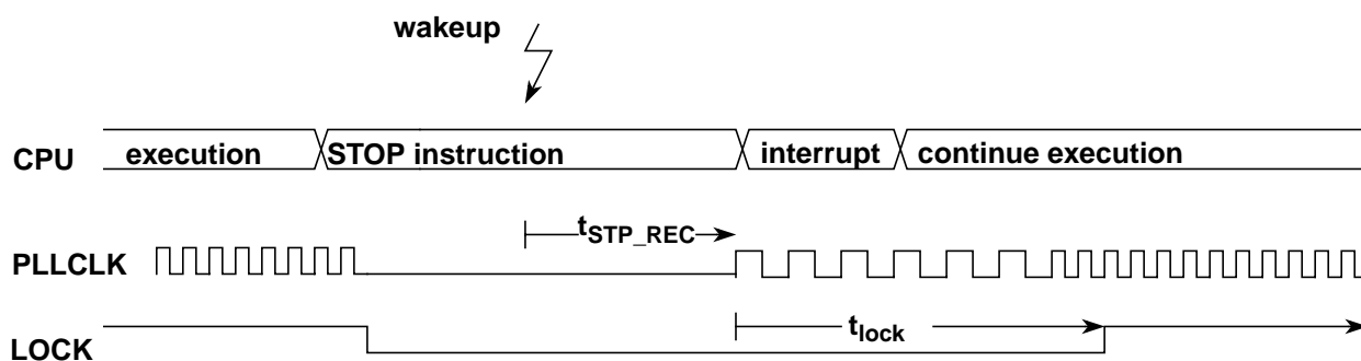
Figure 7-33. Stop Mode using PLL Clock as Bus Clock
