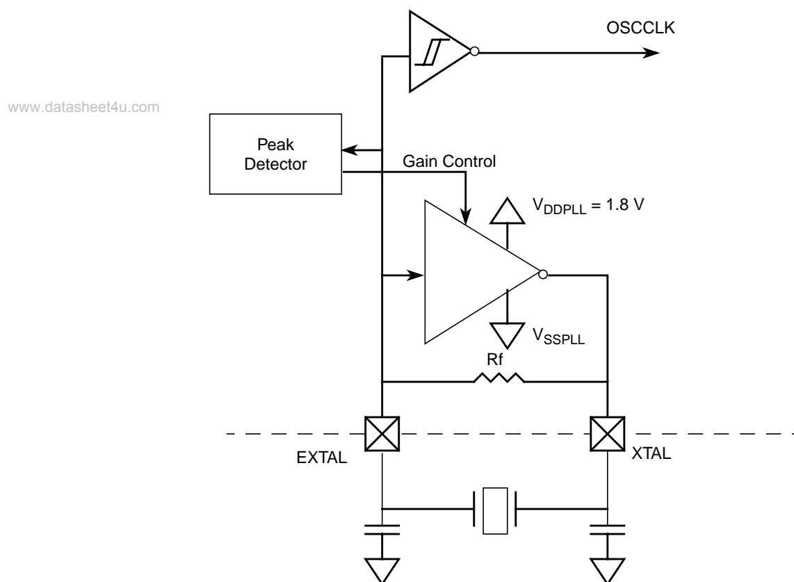
Figure 7-2. OSCLCP Block Diagram
