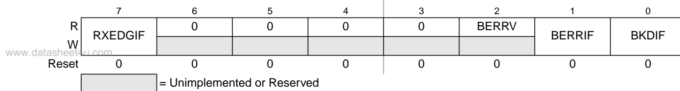
Figure 11-6. SCI Alternative Status Register 1 (SCIASR1)
