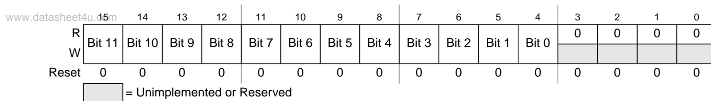
Figure 9-14. Left justified ATD conversion result register (ATDDR n )
