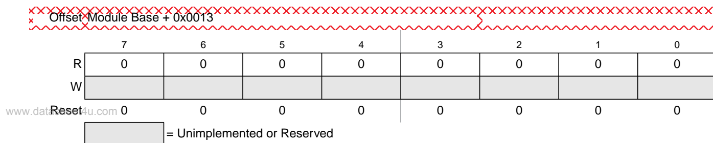
Figure 13-25. Flash Reserved7 Register (FRSV7)
