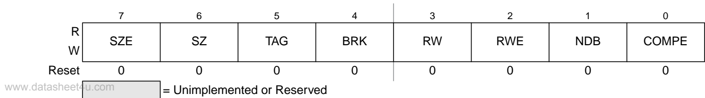
Figure 6-13. Debug Comparator Control Register DBGACTL (Comparator A)
