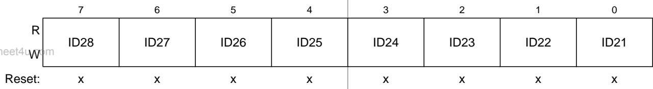
Figure 8-26. Identifier Register 0 (IDR0) — Extended Identifier Mapping
