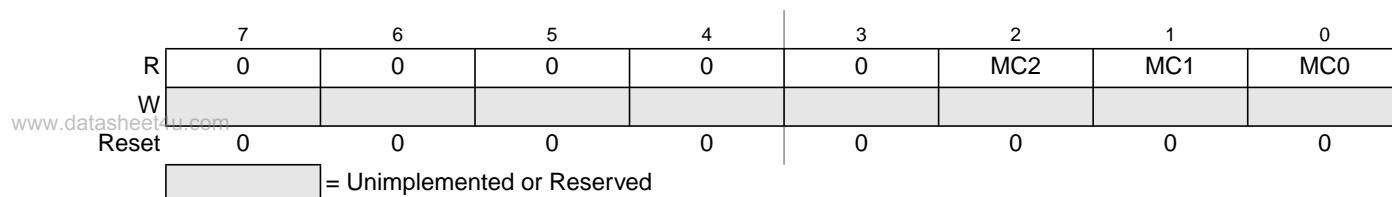
Figure 6-12. Debug Match Flag Register (DBGMFR)
