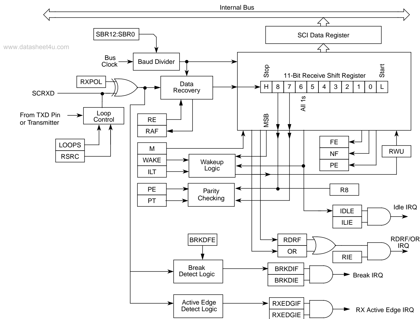
Figure 11-20. SCI Receiver Block Diagram
