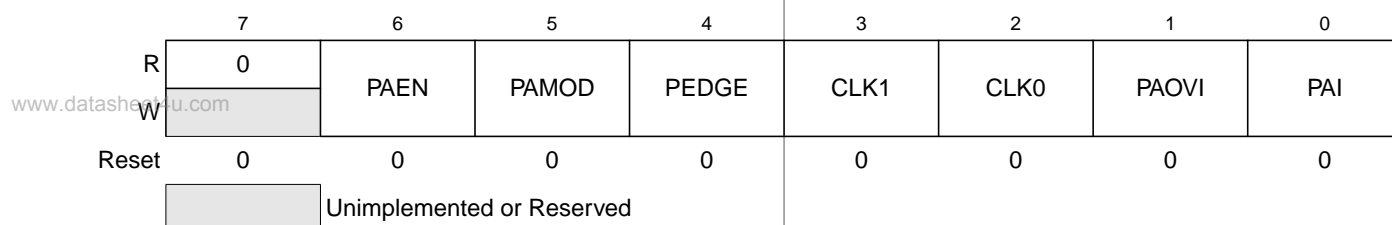
Figure 14-24. 16-Bit Pulse Accumulator Control Register (PACTL)
