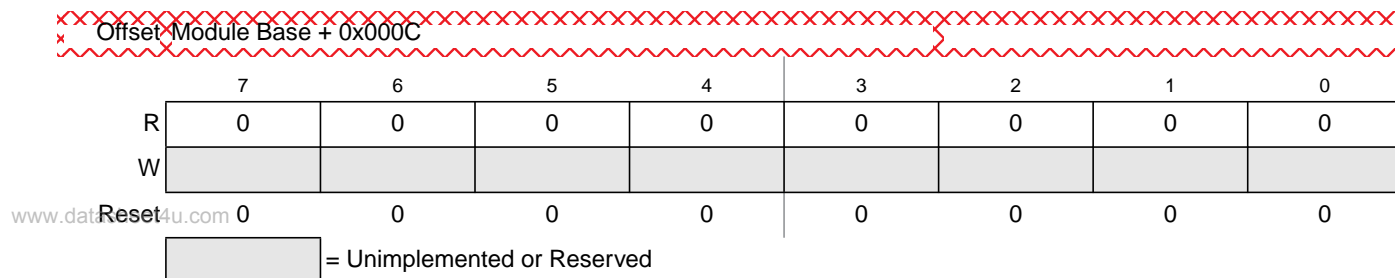
Figure 13-20. Flash Reserved3 Register (FRSV3)
