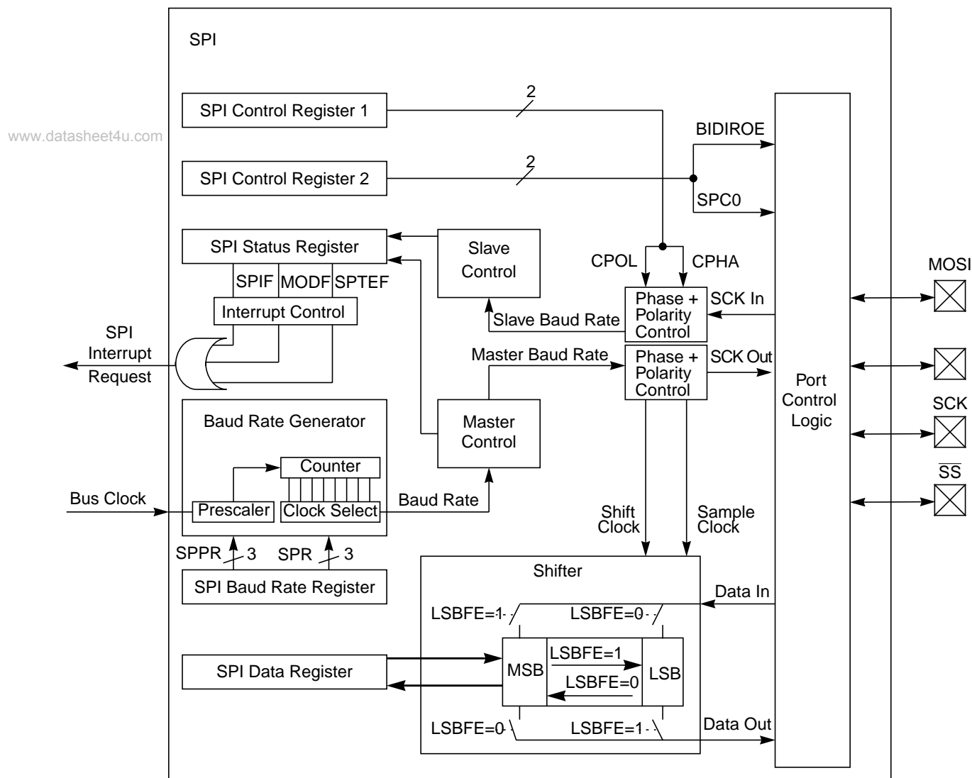
Figure 12-1. SPI Block Diagram
