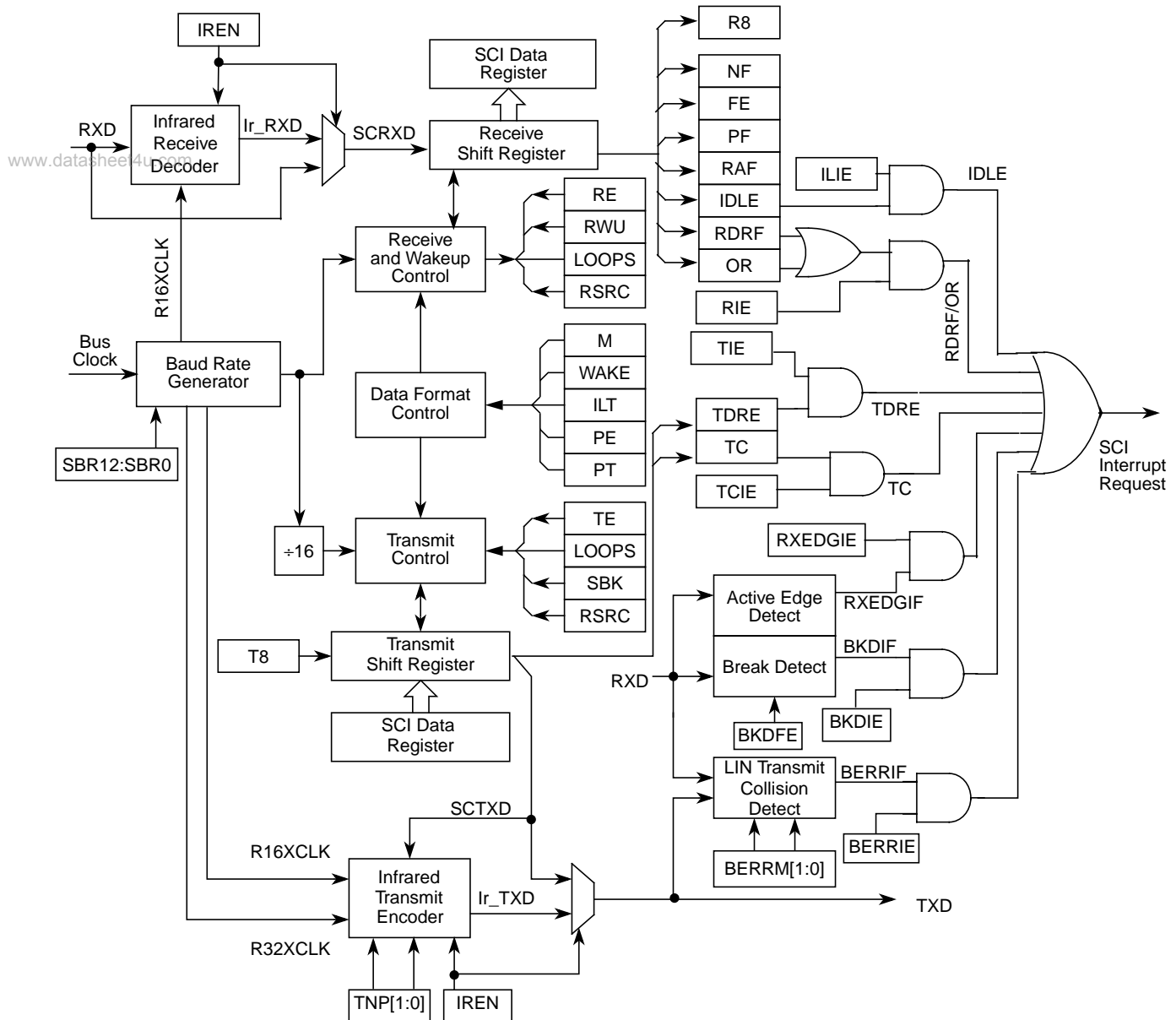
Figure 11-14. Detailed SCI Block Diagram
