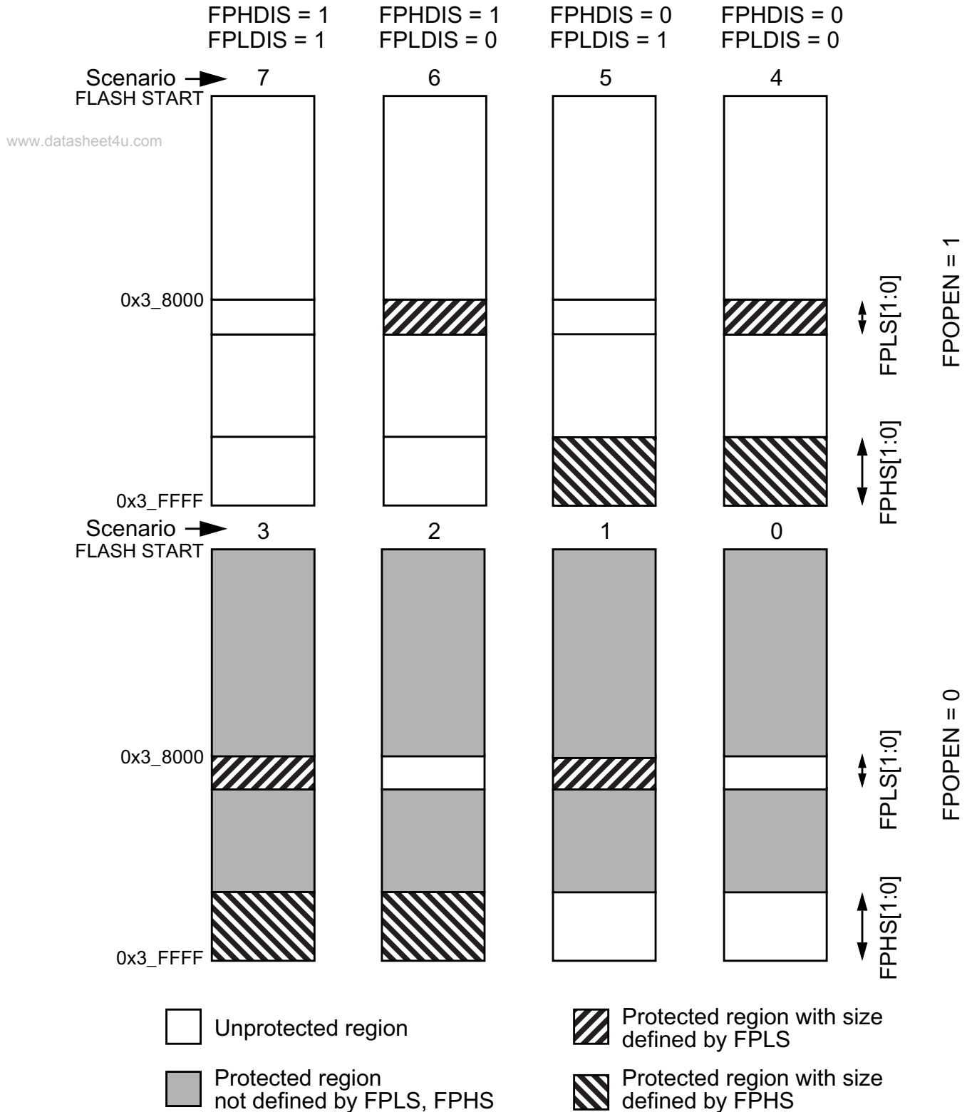
Figure 13-14. P-Flash Protection Scenarios
