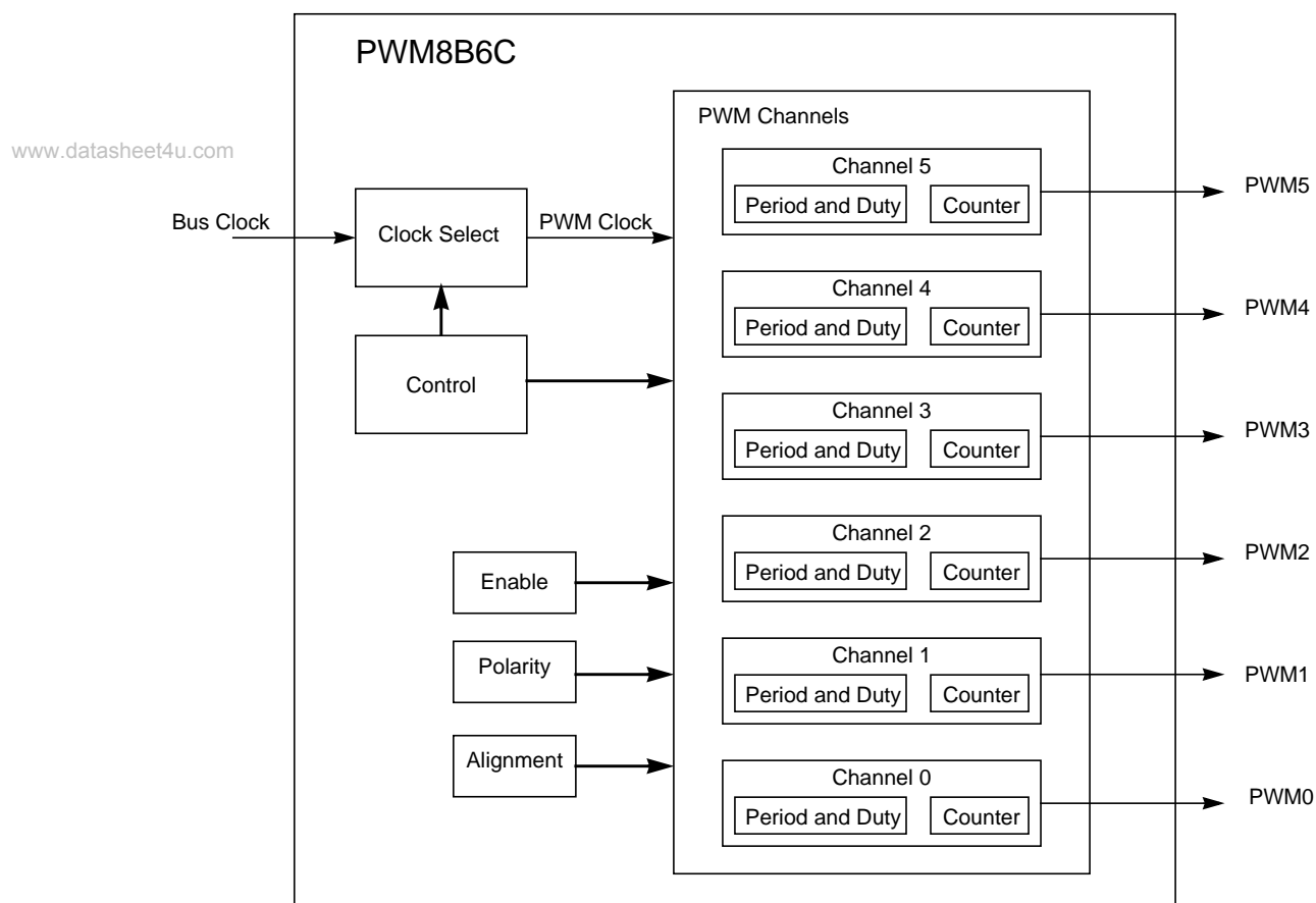
Figure 10-1. PWM8B6CV1 Block Diagram
