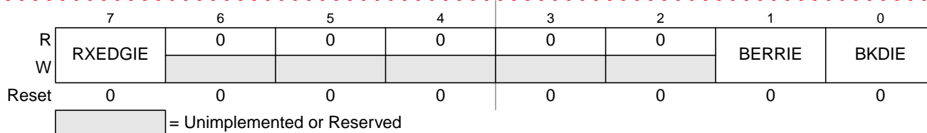
Figure 11-7. SCI Alternative Control Register 1 (SCIACR1)
