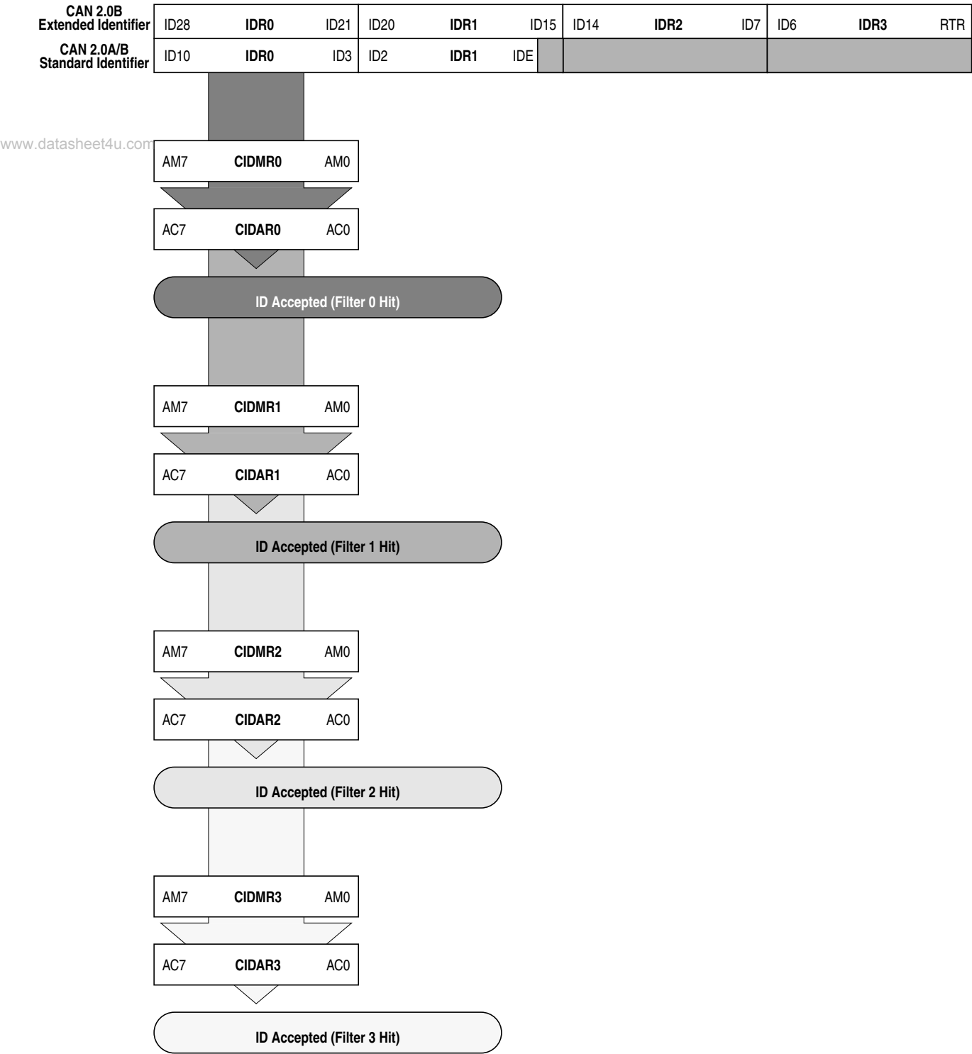
Figure 8-42. 8-bit Maskable Identifier Acceptance Filters
