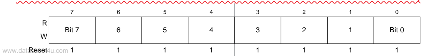
Figure 10-32. PWM Channel Duty Registers (PWMDTY5)
