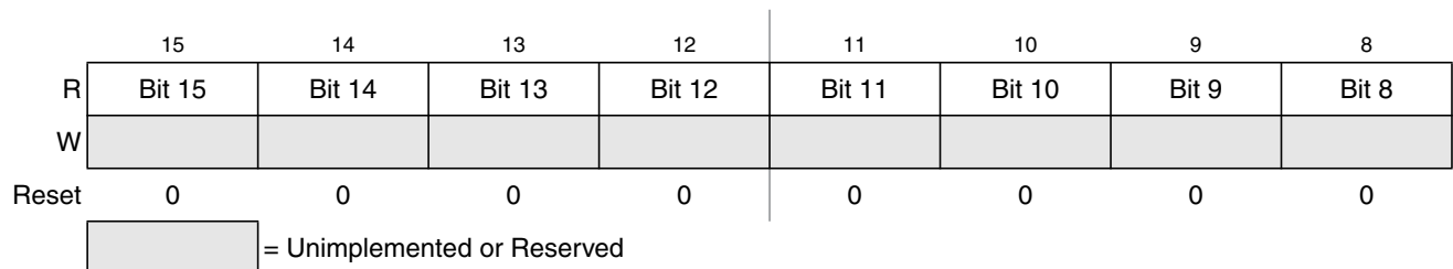
Figure 18-11. Debug Comparator C Register High (DBG CCH)
