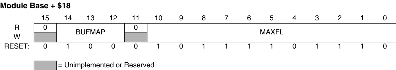
Figure 11-16. Ethernet Buffer Configuration (BUFCFG)
