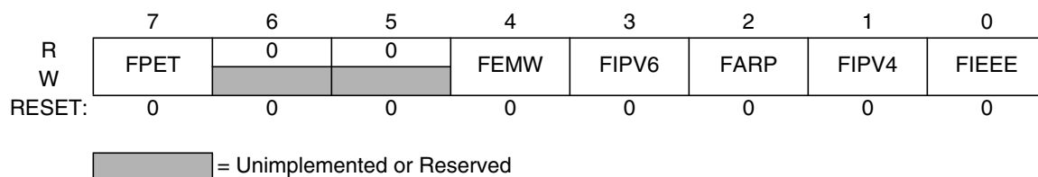
Figure 11-5. Ethertype Control (ETCTL)
