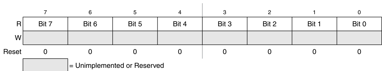
Figure 18-12. Debug Comparator C Register Low (DBG CCL)
