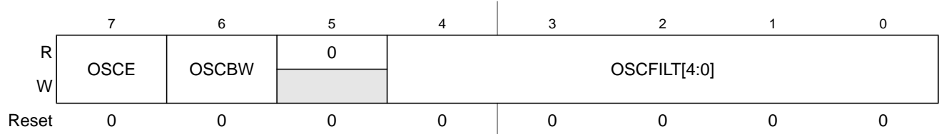
Figure 7-28. S12CPMU Oscillator Register (CPMUOSC)
