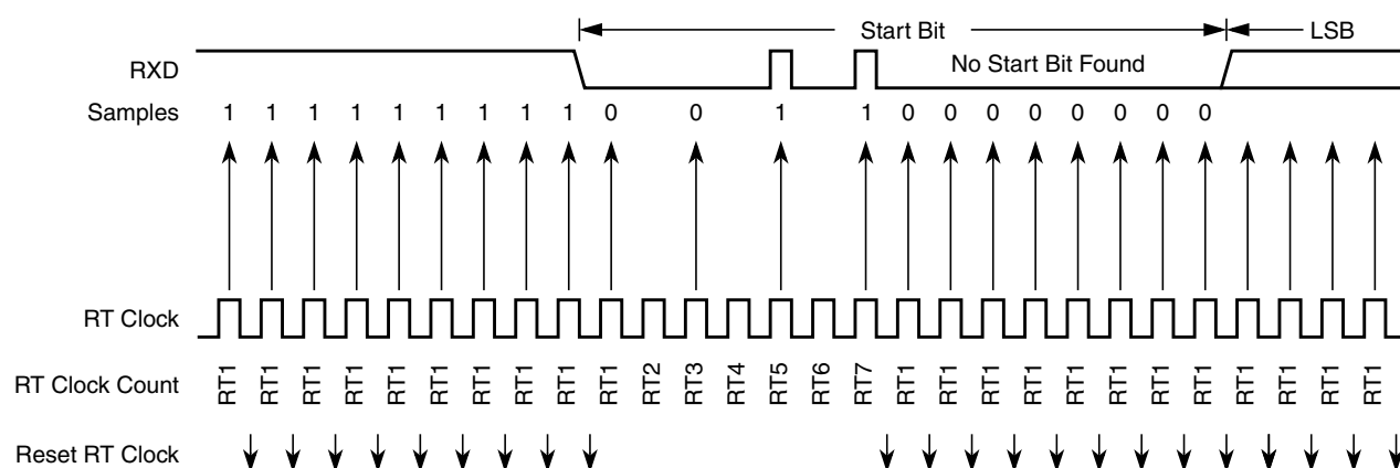
Figure 18-26. Start Bit Search Example 5
