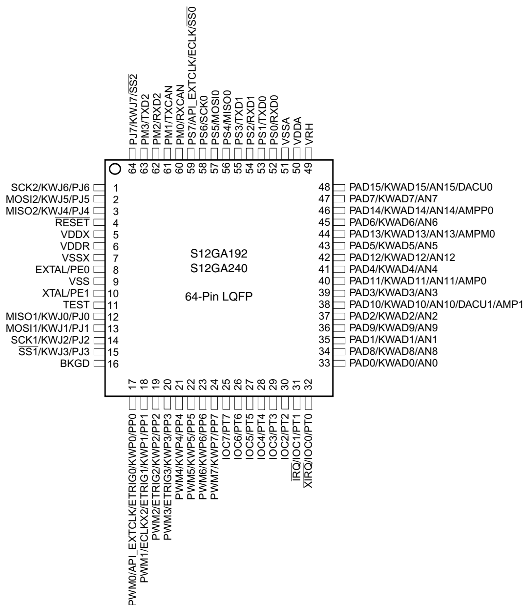
Figure 1-19. 64-Pin LQFP Pinout for S12GA192 and S12GA240
