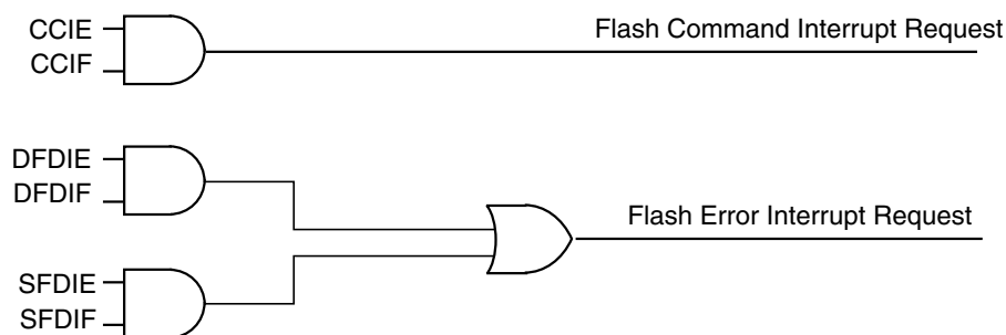
Figure 22-27. Flash Module Interrupts Implementation
