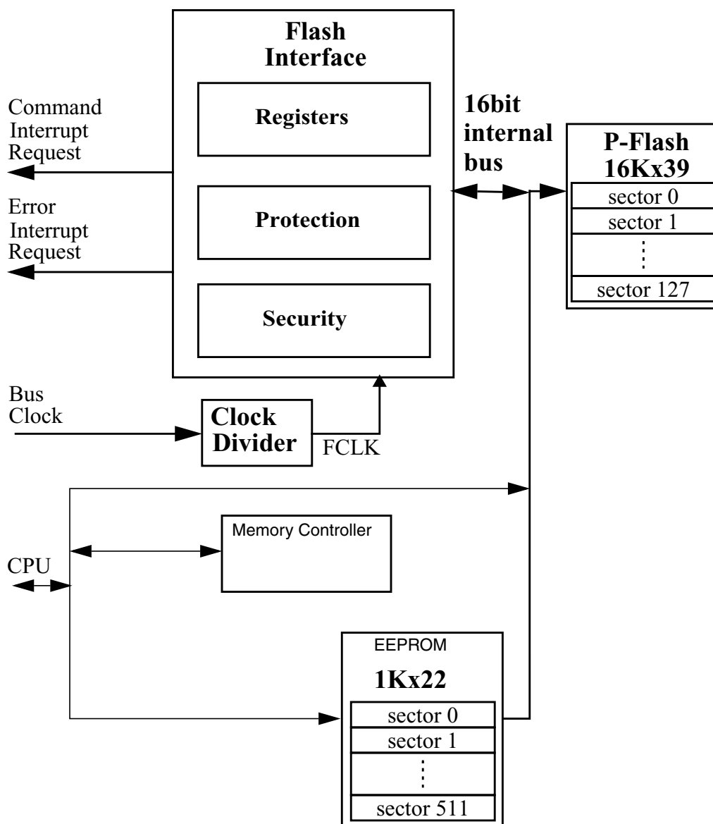
Figure 24-1. FTMRG64K1 Block Diagram
