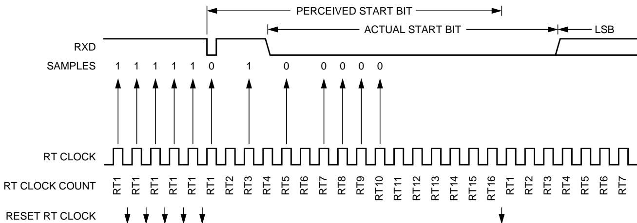
In Figure 8-17 , verification sample at RT3 is high. The RT3 sample sets the noise flag. Although the perceived bit time is misaligned, the data samples RT8, RT9, and RT10 are within the bit time and data recovery is successful.
