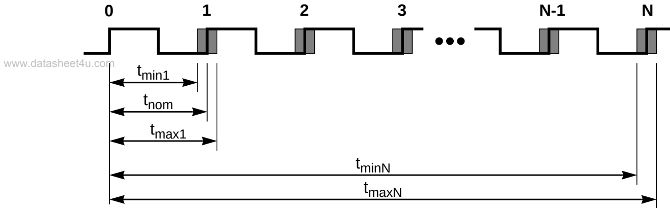
Figure A-3 Jitter Definitions
