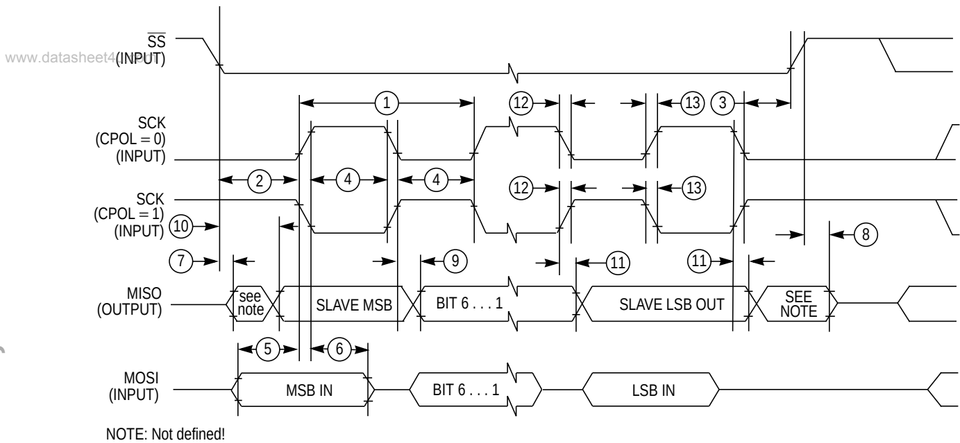
Figure A-7 SPI Slave Timing (CPHA=0)
