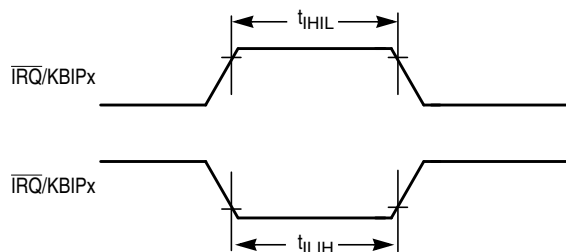
Figure 10. \overline{\text{IRQ}}/\text{KBIPx} Timing
